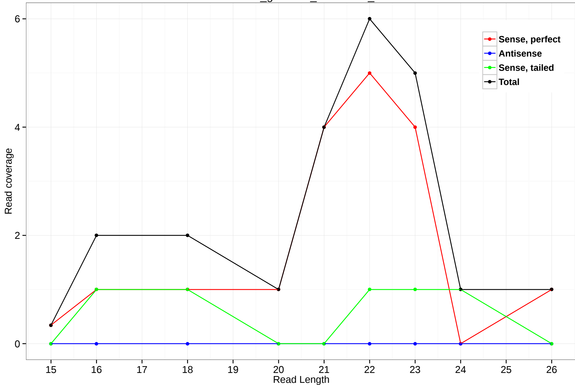
rheMac3_genscan_chr9.2025_50
