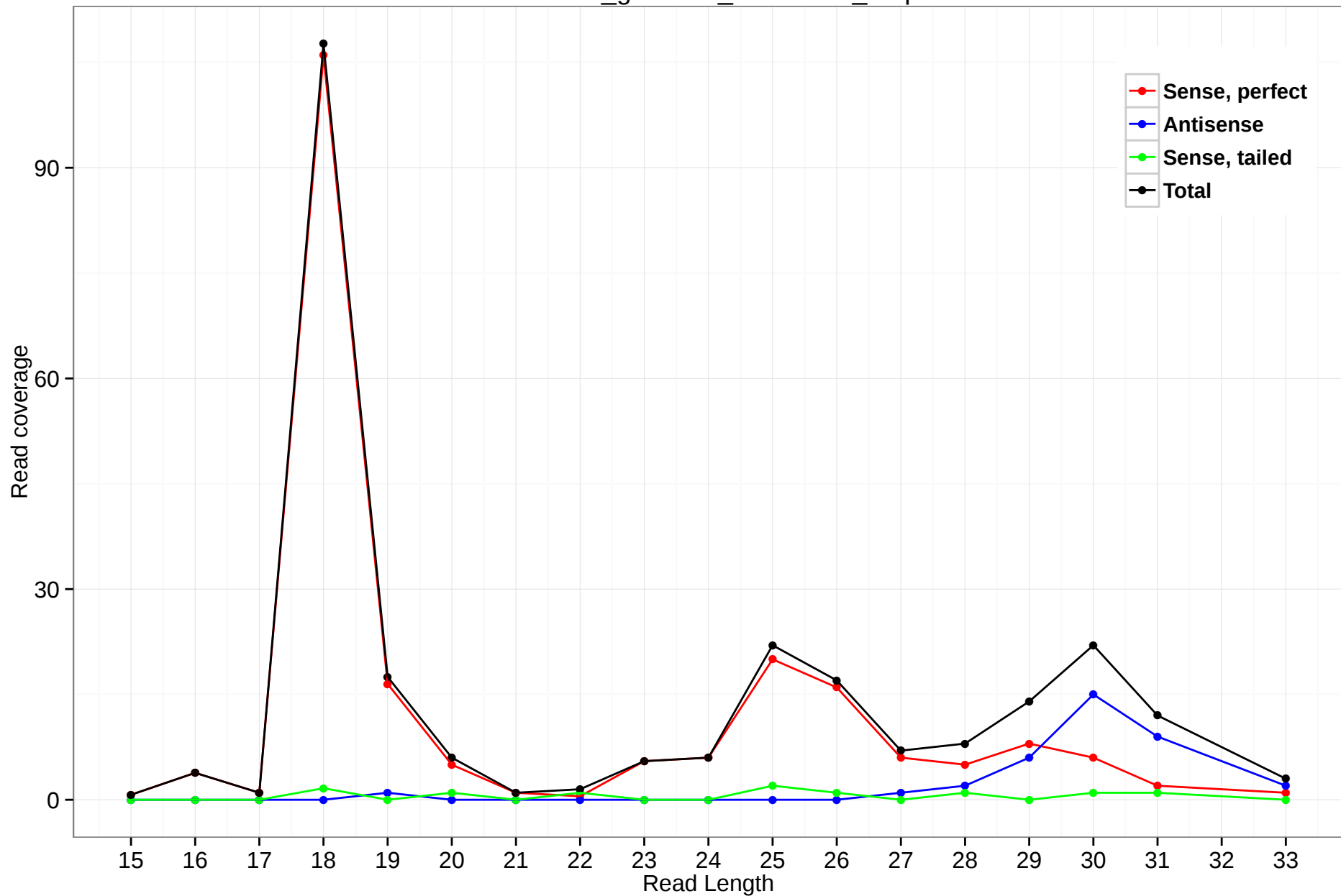
rheMac3_genscan_chr9.1980_0.3p
