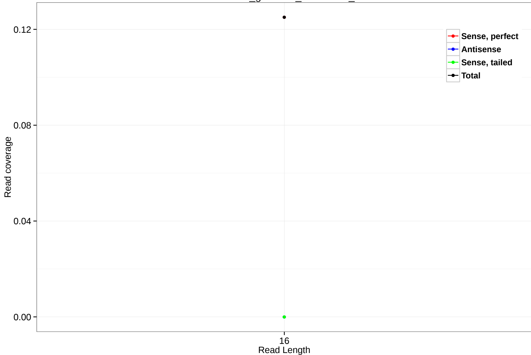
rheMac3_genscan_chr9.1919_5
