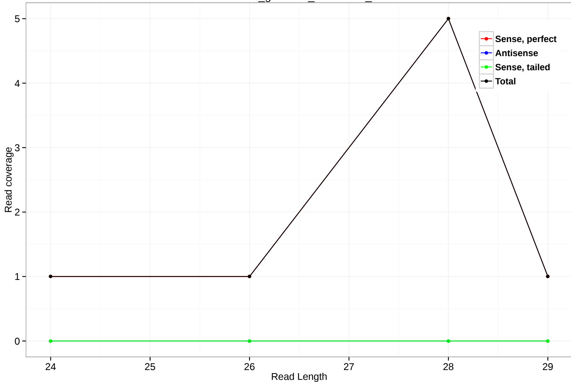
rheMac3_genscan_chr9.1854_15
