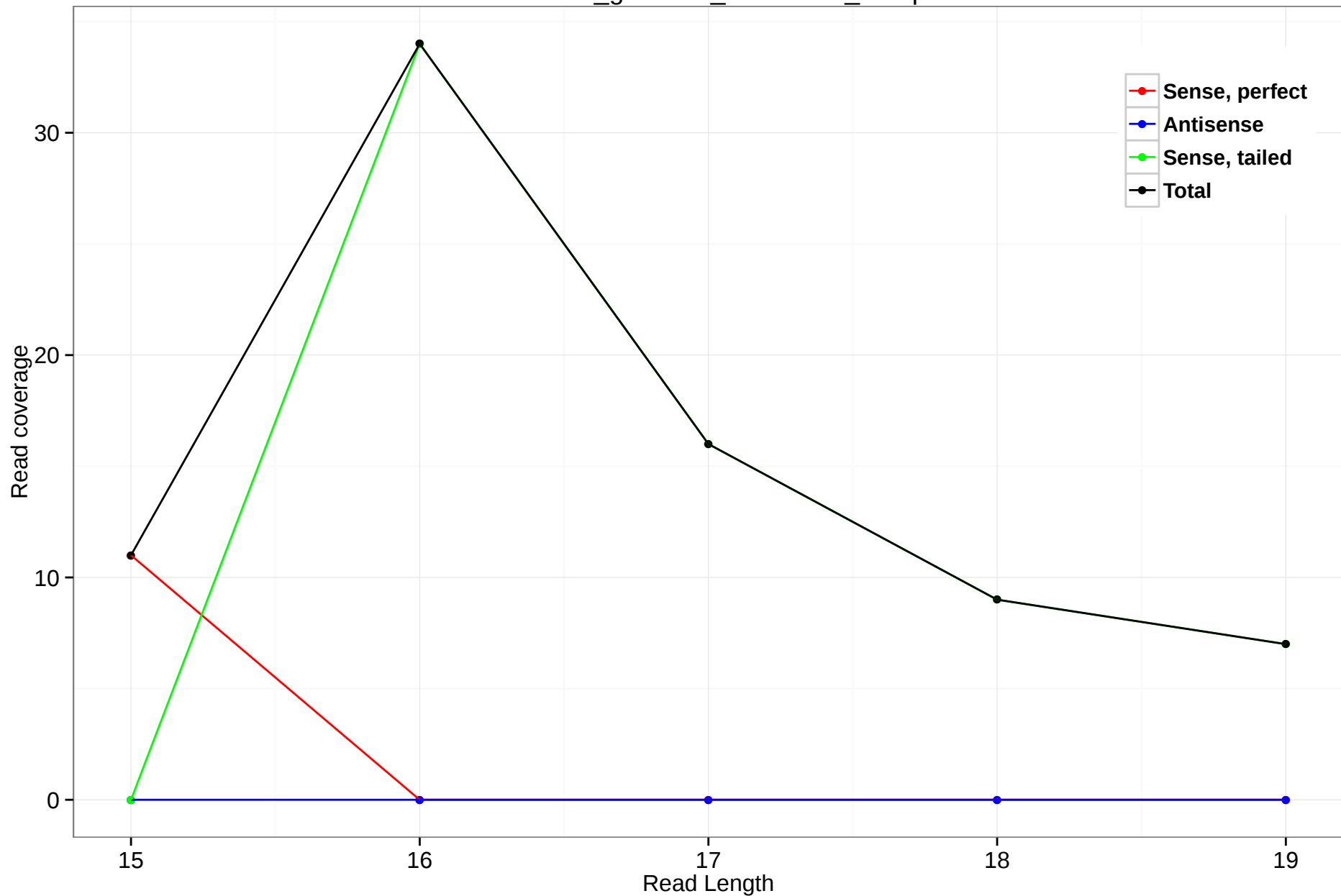
rheMac3_genscan_chr9.1816_34.3p
