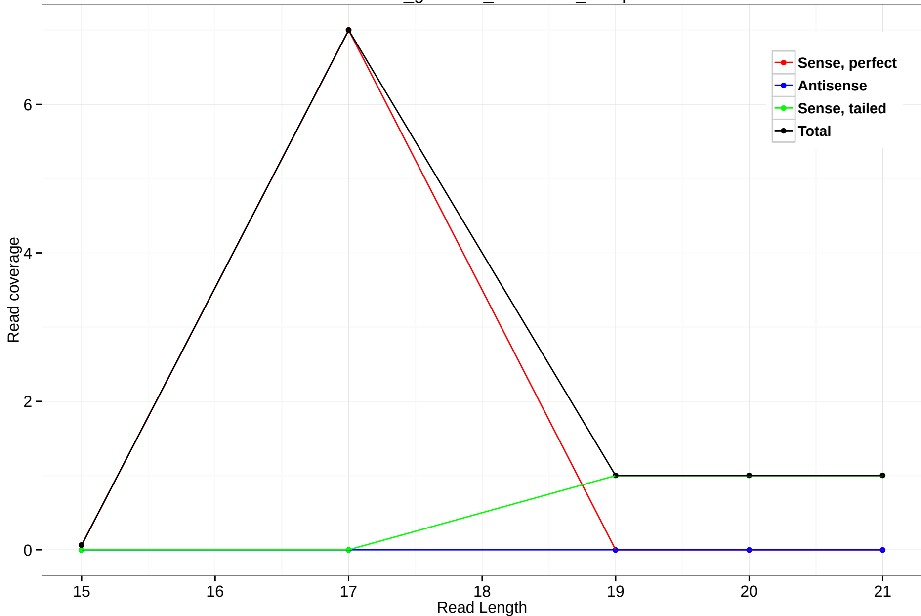
rheMac3_genscan_chr9.1816_30.3p
