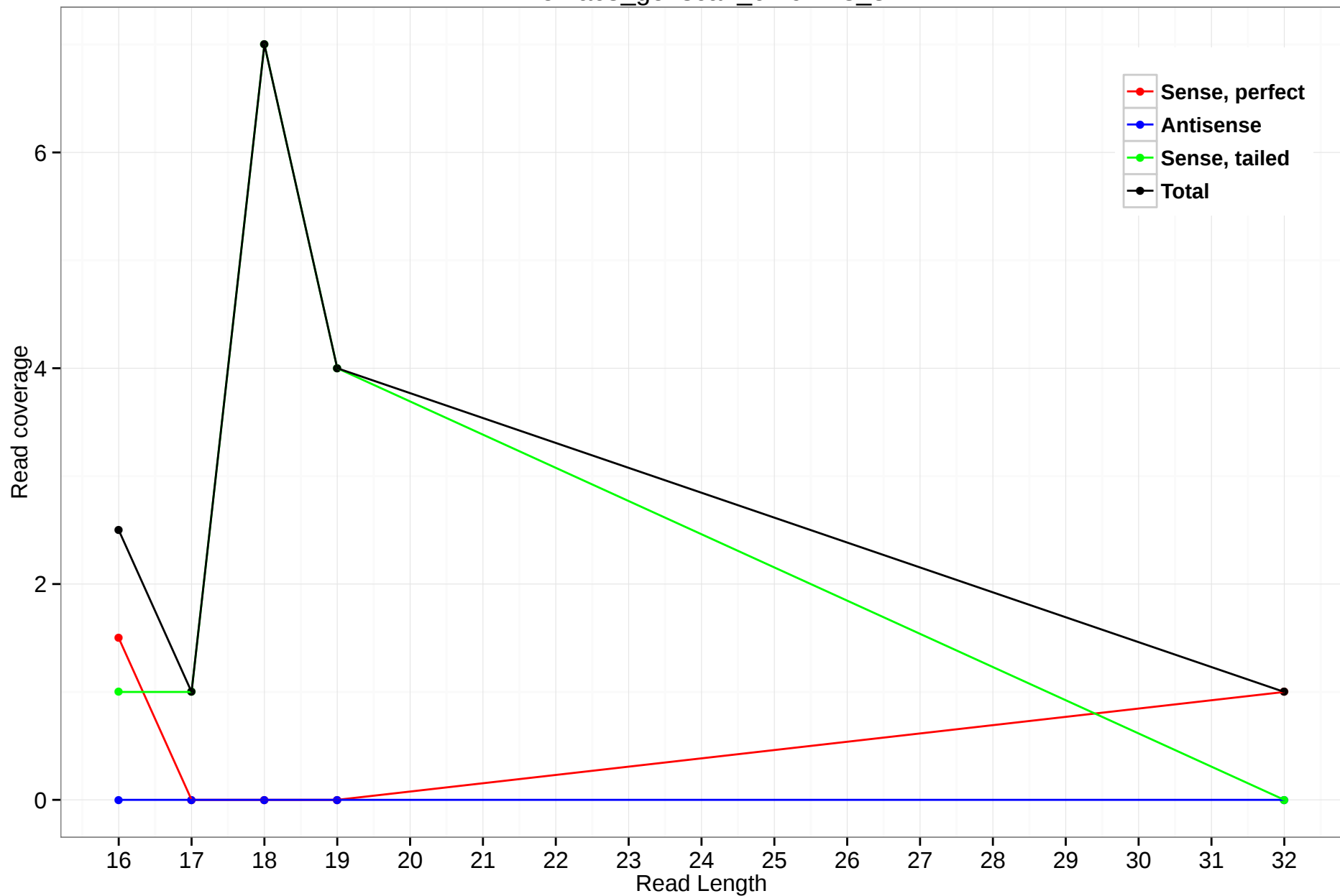
rheMac3_genscan_chr9.178_3
