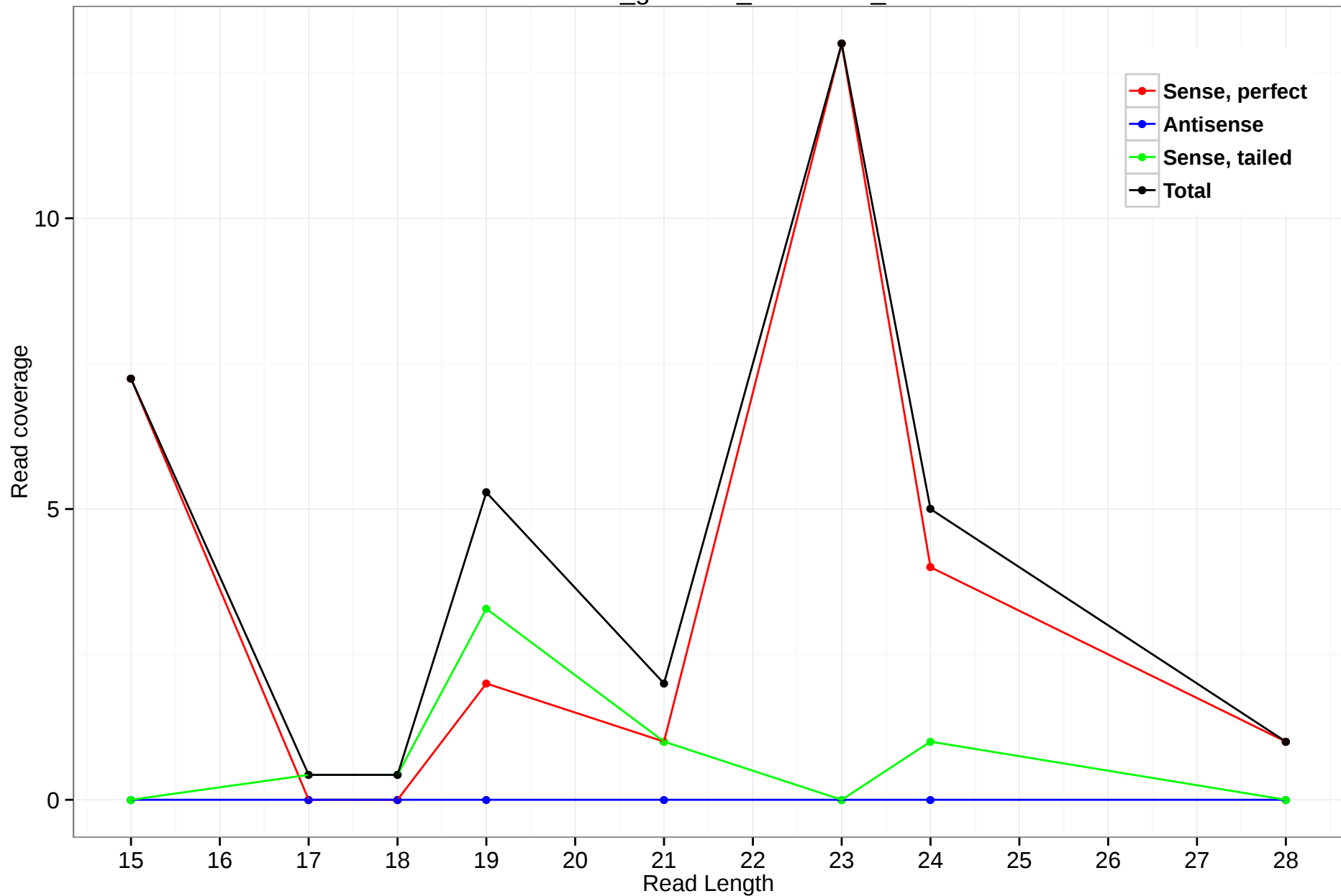
rheMac3_genscan_chr9.1738_7
