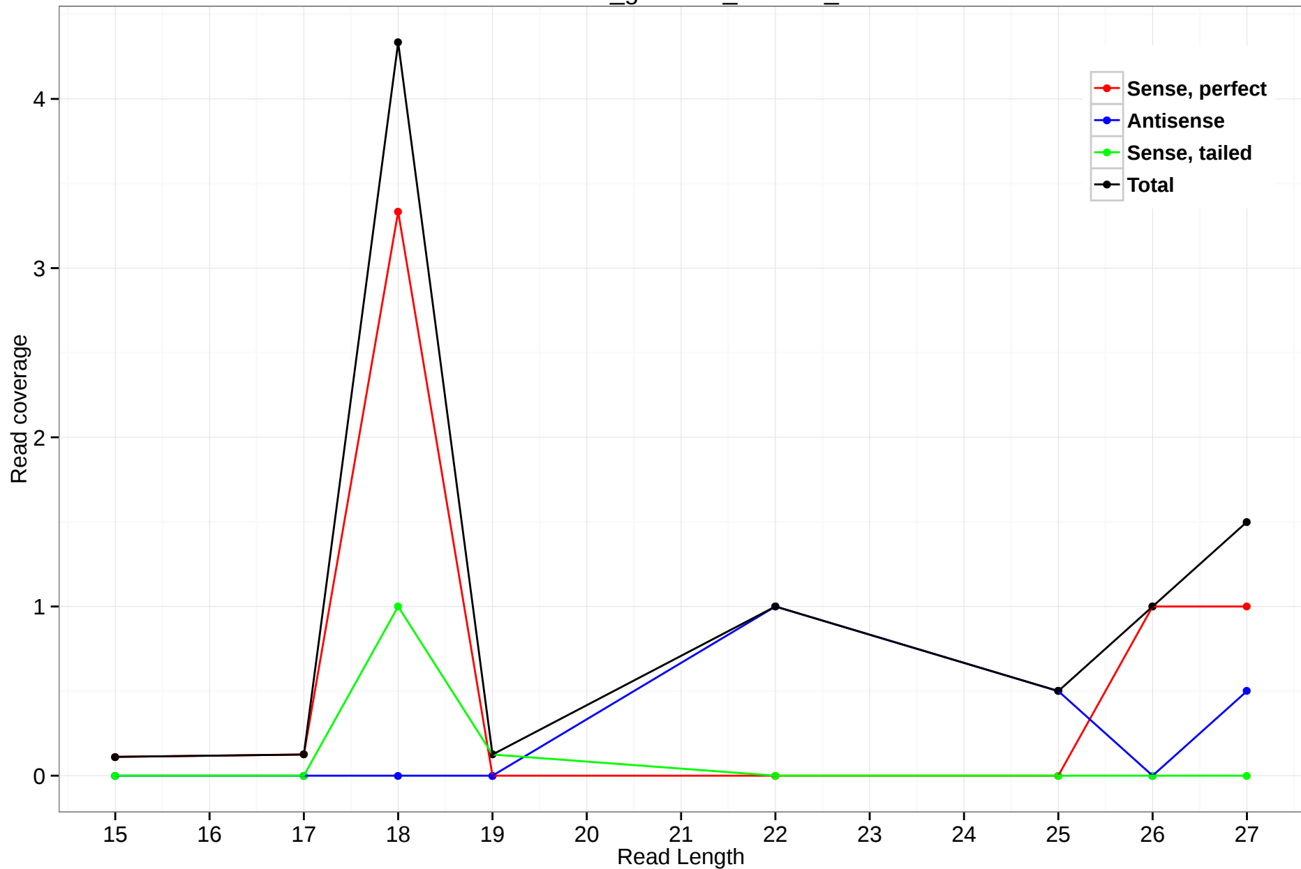
rheMac3_genscan_chr9.14_0
