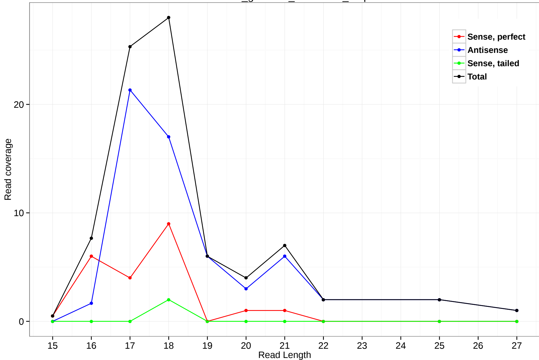
rheMac3_genscan_chr9.1446_0.5p
