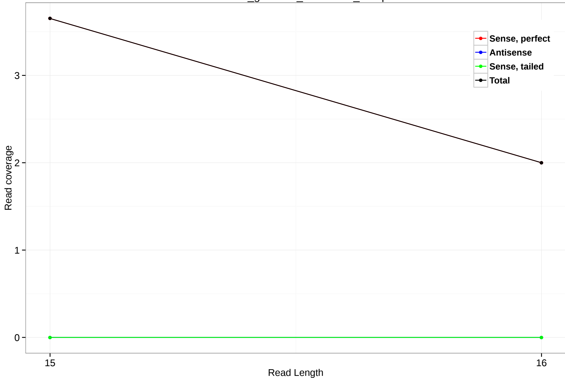
rheMac3_genscan_chr9.1445_16.3p
