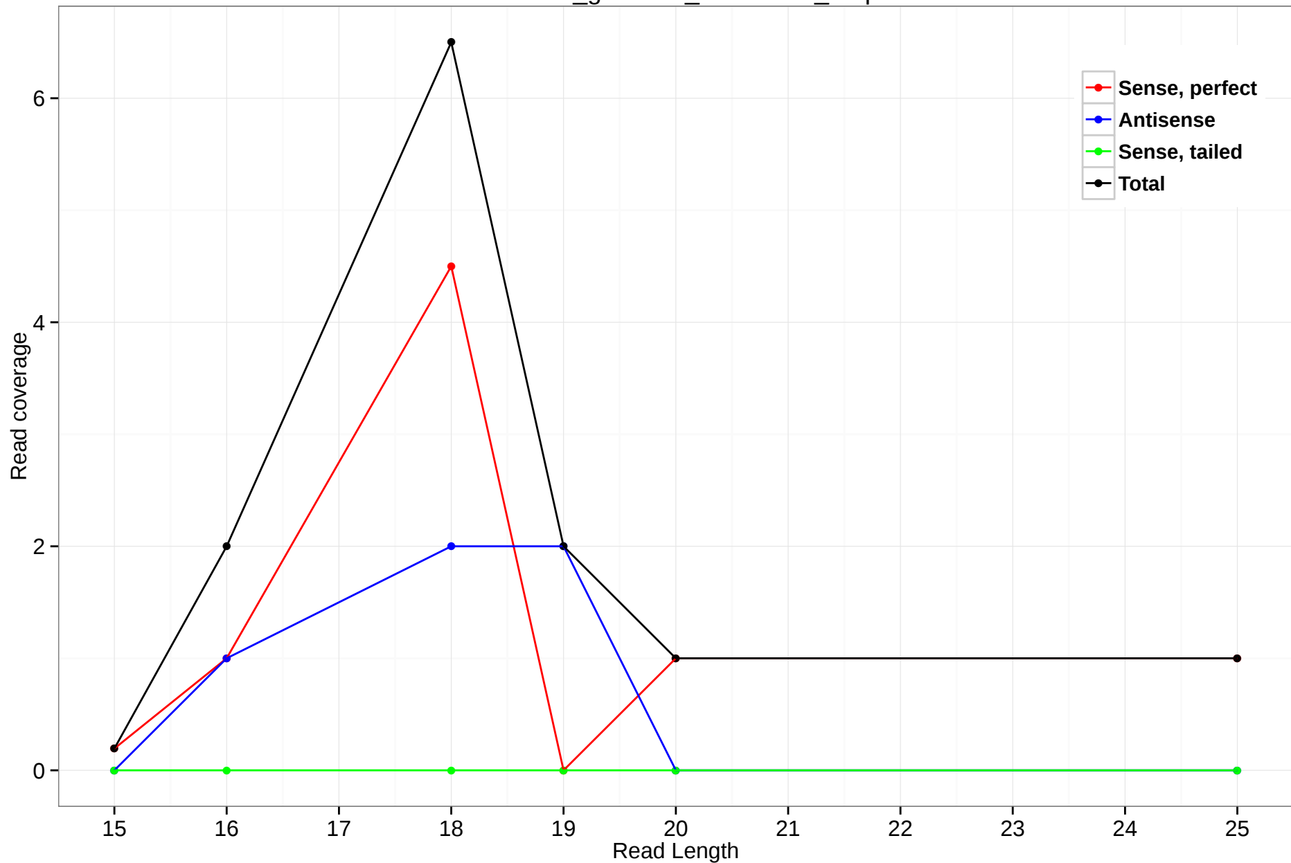
rheMac3_genscan_chr9.1443_1.5p
