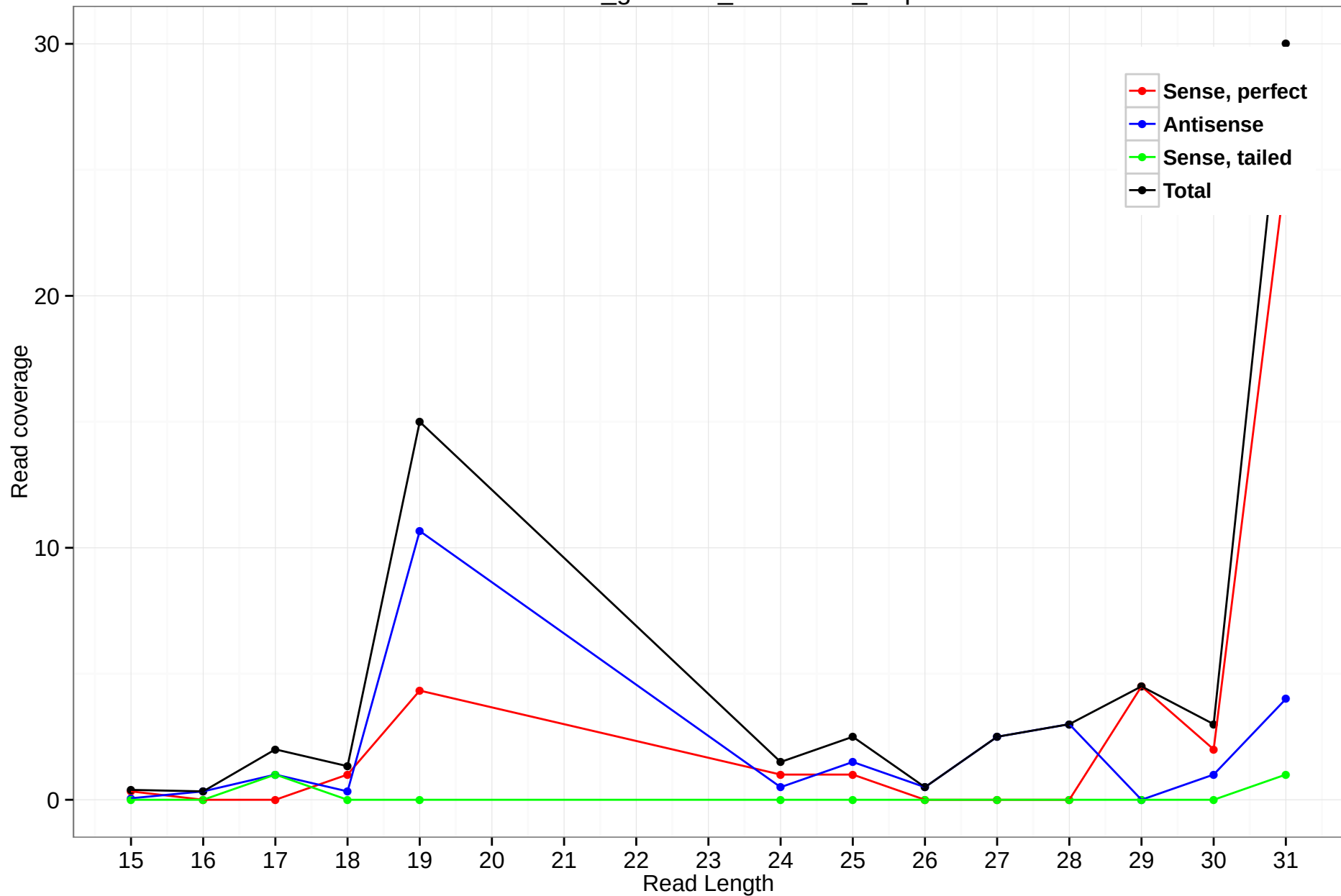
rheMac3_genscan_chr9.1406_7.3p
