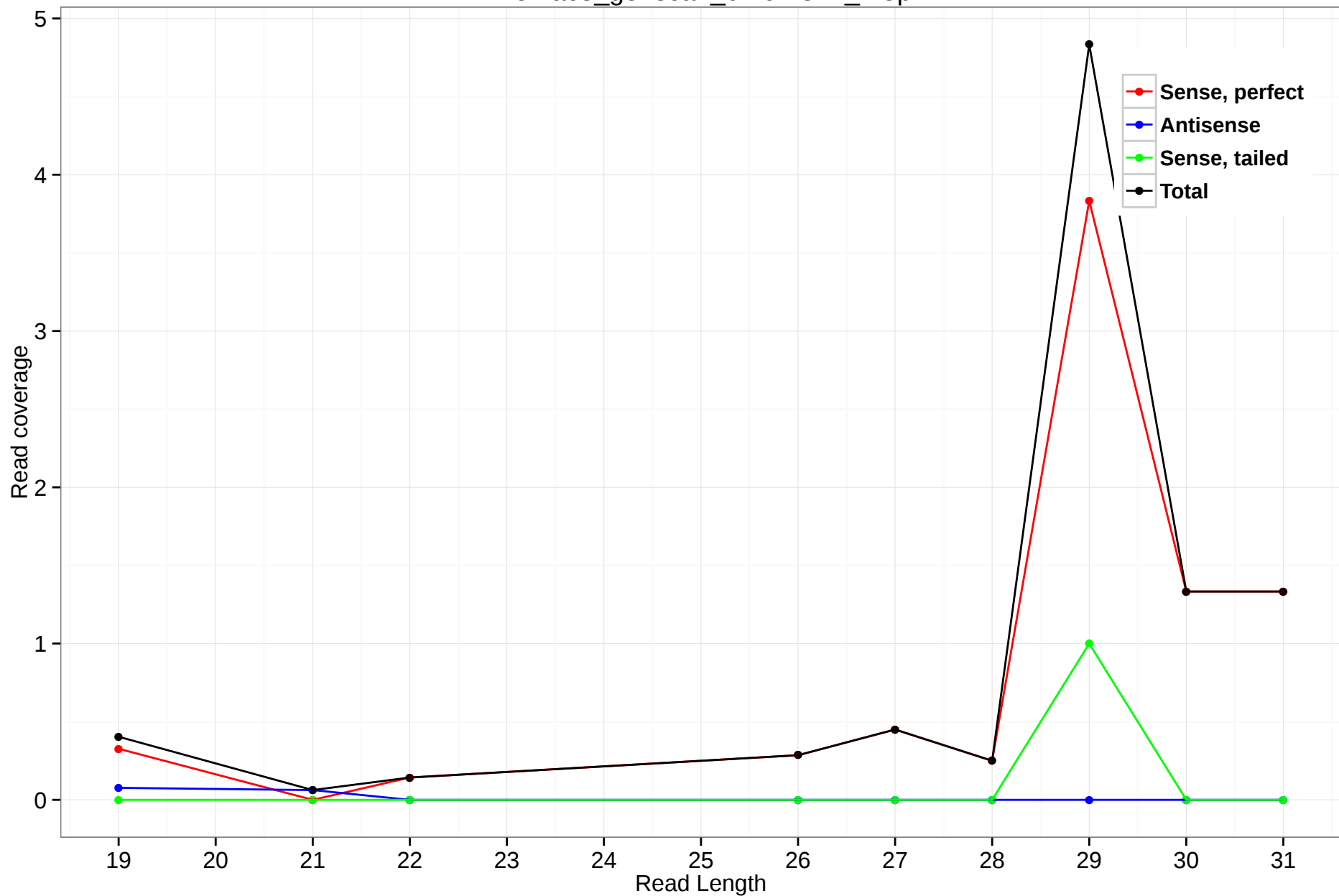
rheMac3_genscan_chr9.1377_2.5p
