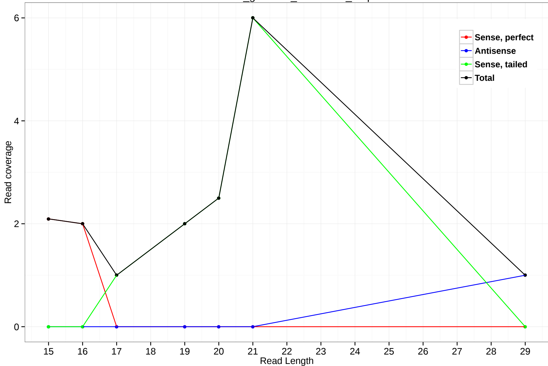
rheMac3_genscan_chr9.1367_5.3p
