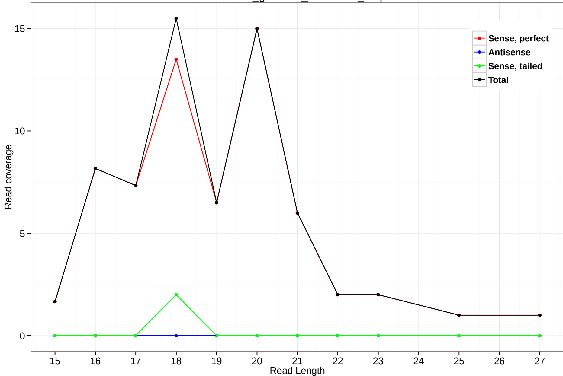
rheMac3_genscan_chr9.1347_1.3p
