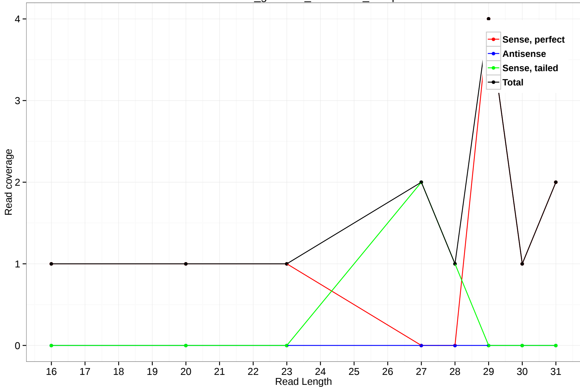
rheMac3_genscan_chr9.1345_12.5p
