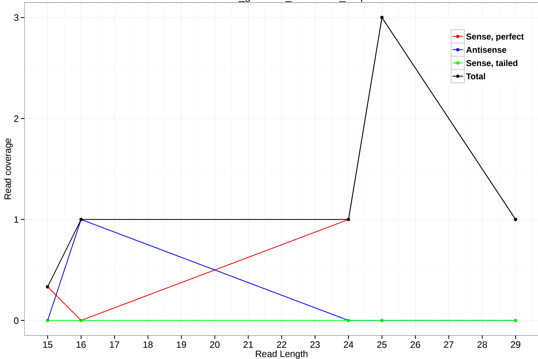
rheMac3_genscan_chr9.1345_0.5p
