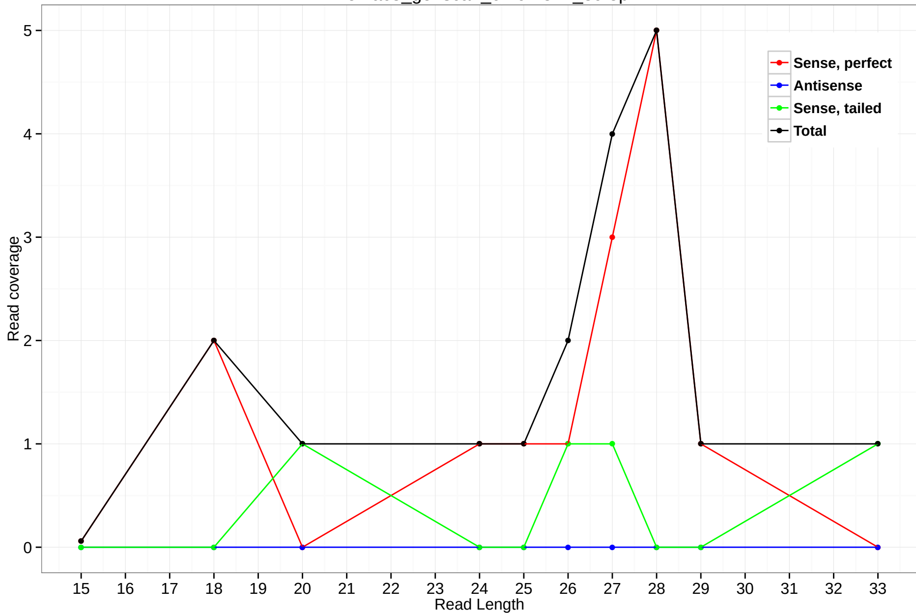
rheMac3_genscan_chr9.1327_39.5p
