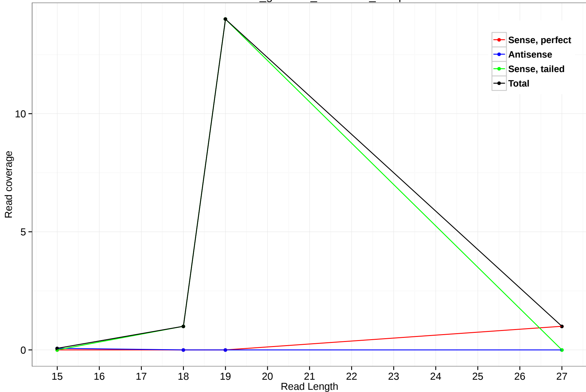
rheMac3_genscan_chr9.1327_14.3p
