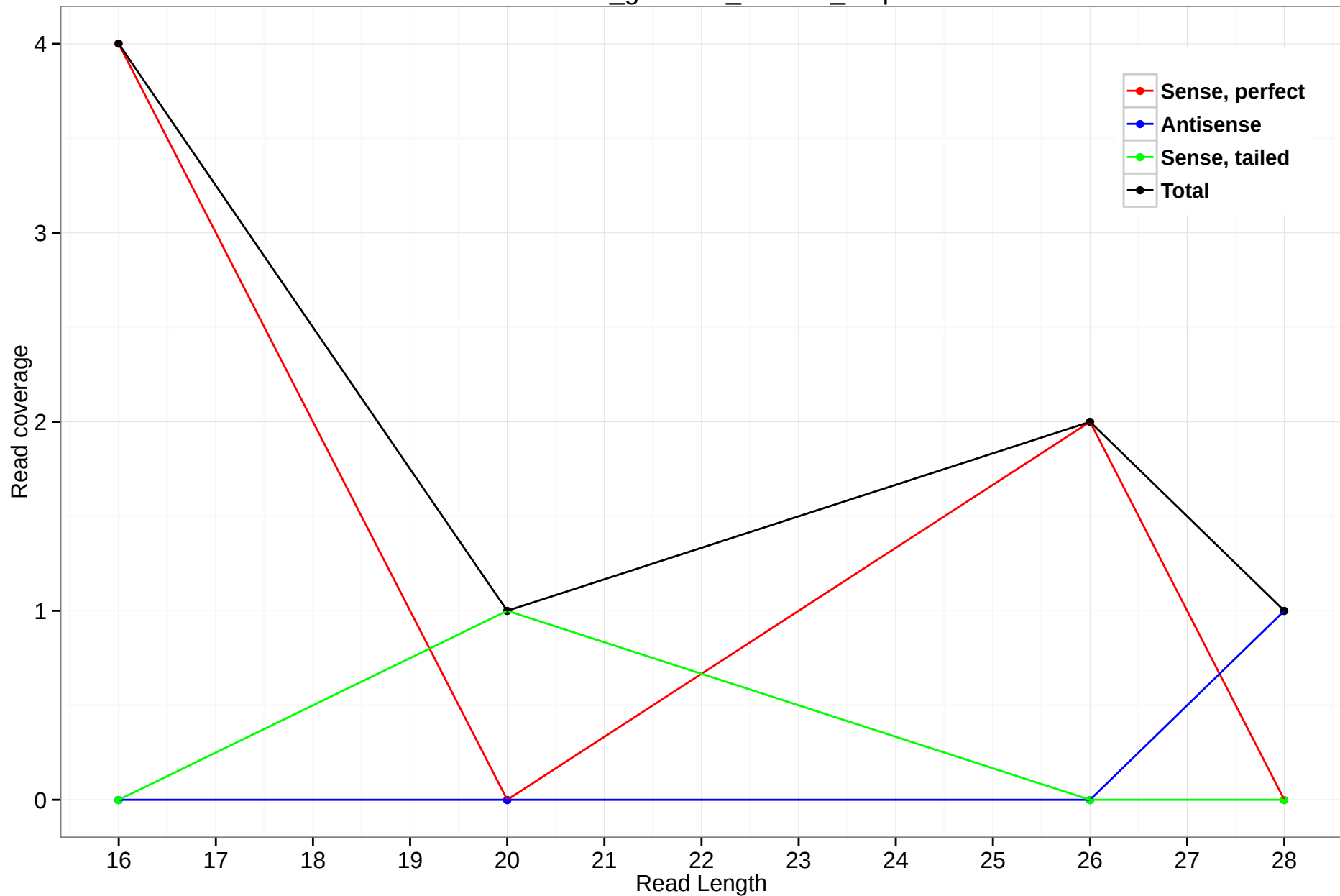
rheMac3_genscan_chr9.12_8.3p
