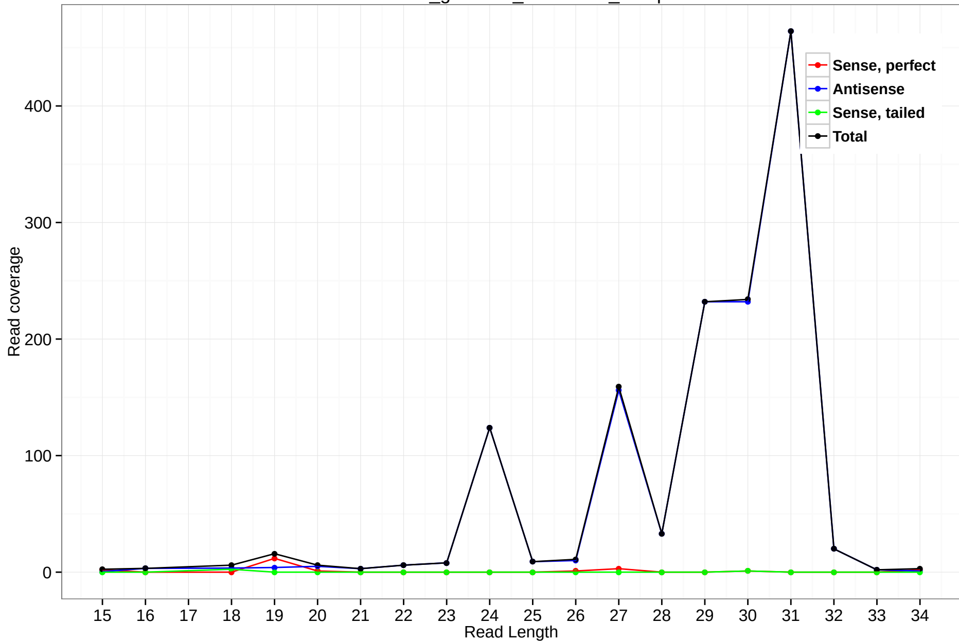
rheMac3_genscan_chr9.1224_40.5p
