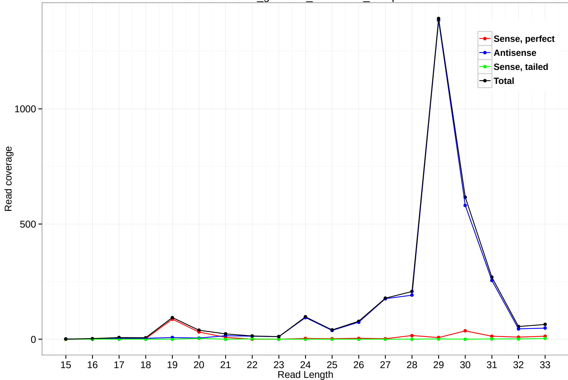
rheMac3_genscan_chr9.1224_40.3p
