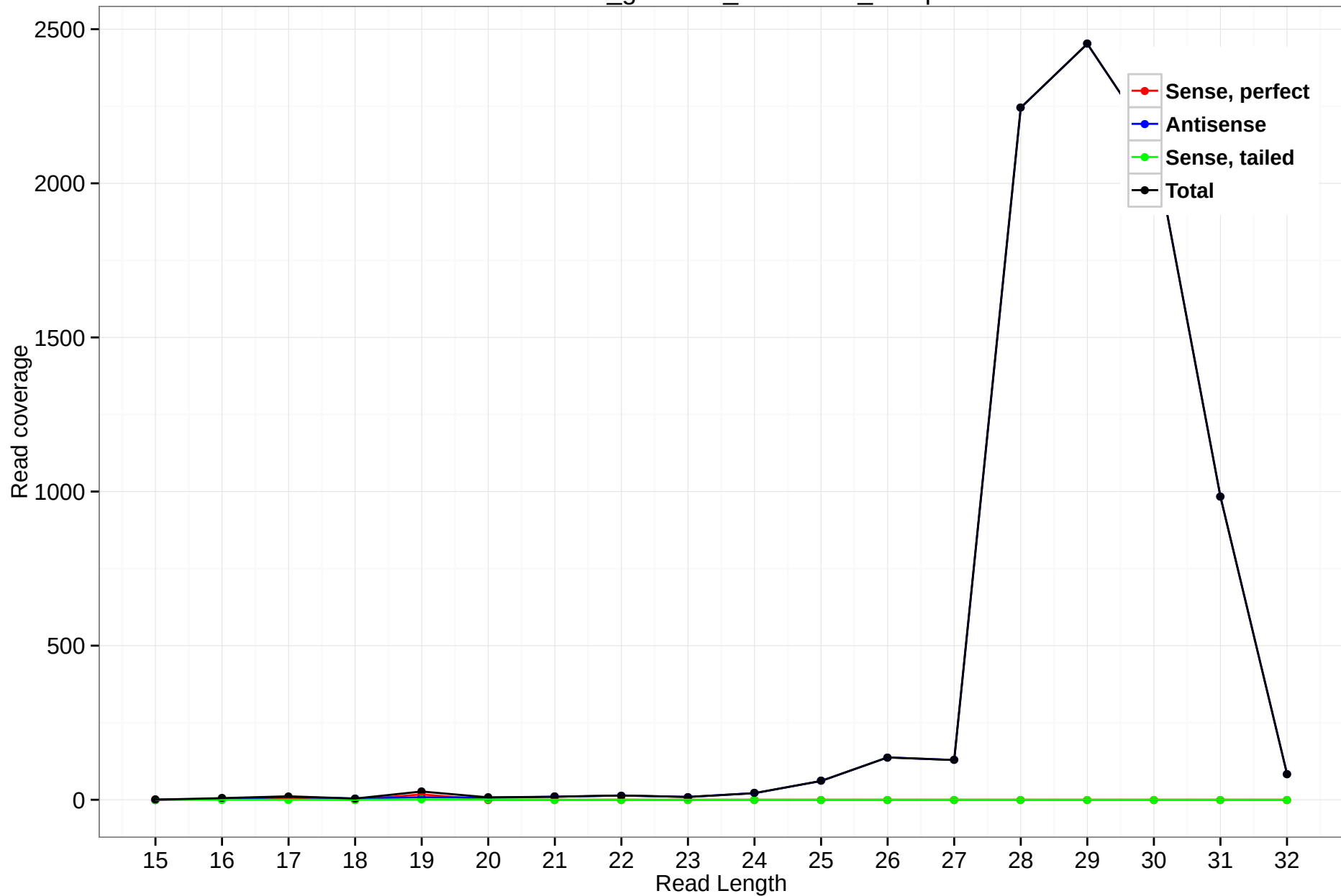
rheMac3_genscan_chr9.1224_38.5p
