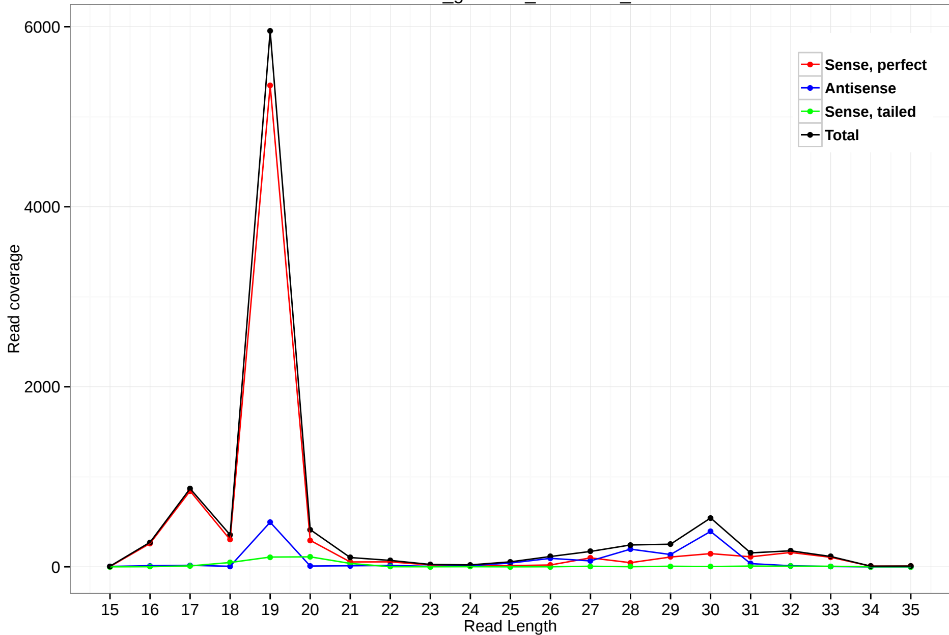
rheMac3_genscan_chr9.1224_34
