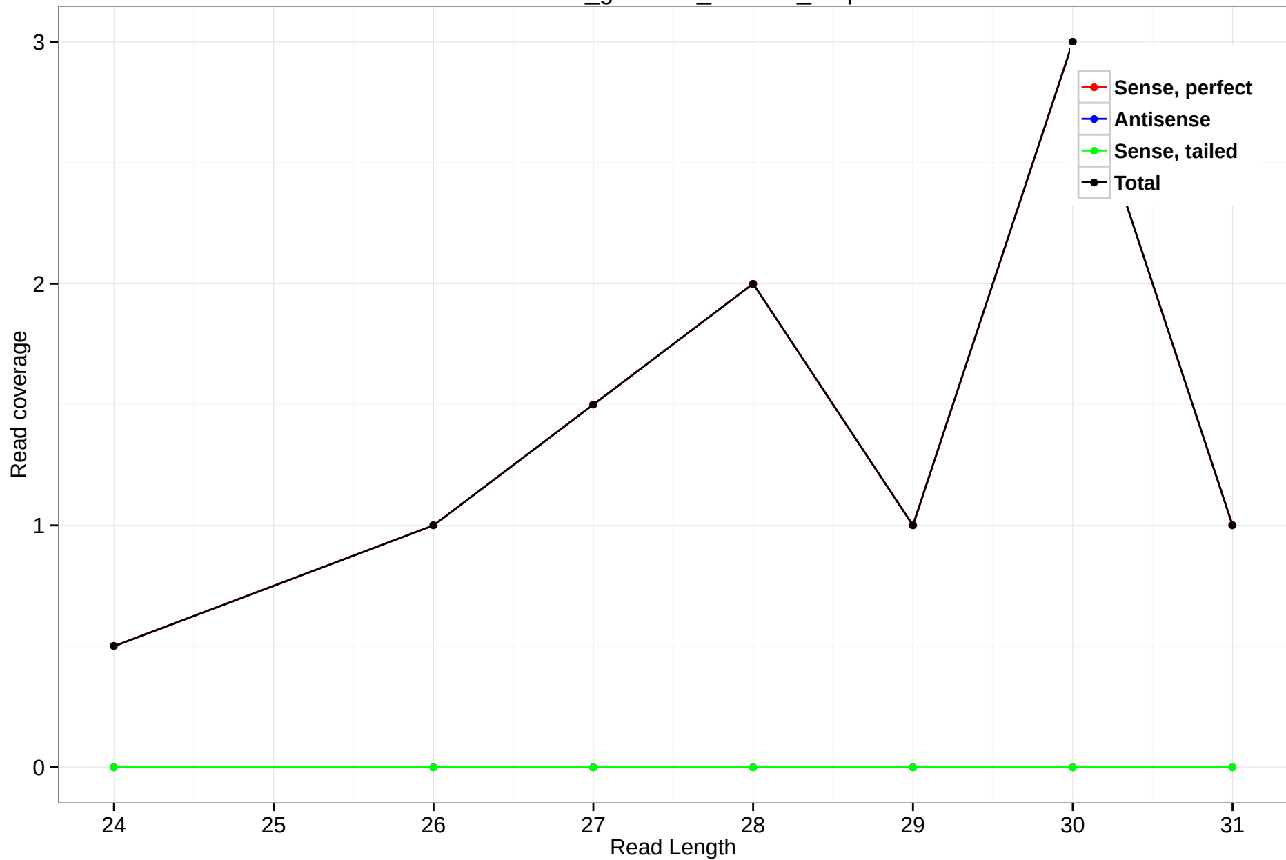
rheMac3_genscan_chr9.11_1.5p
