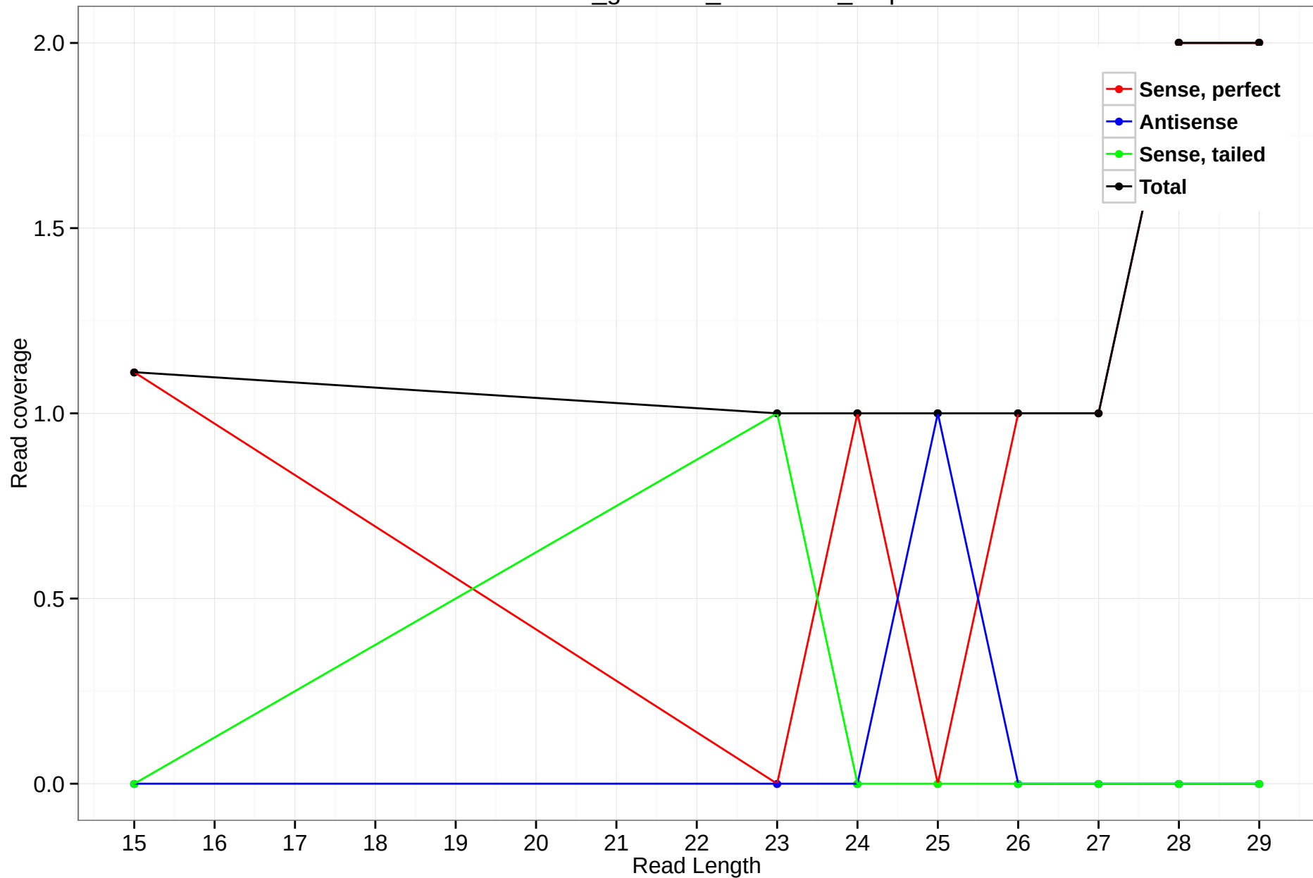
rheMac3_genscan_chr9.1177_5.3p
