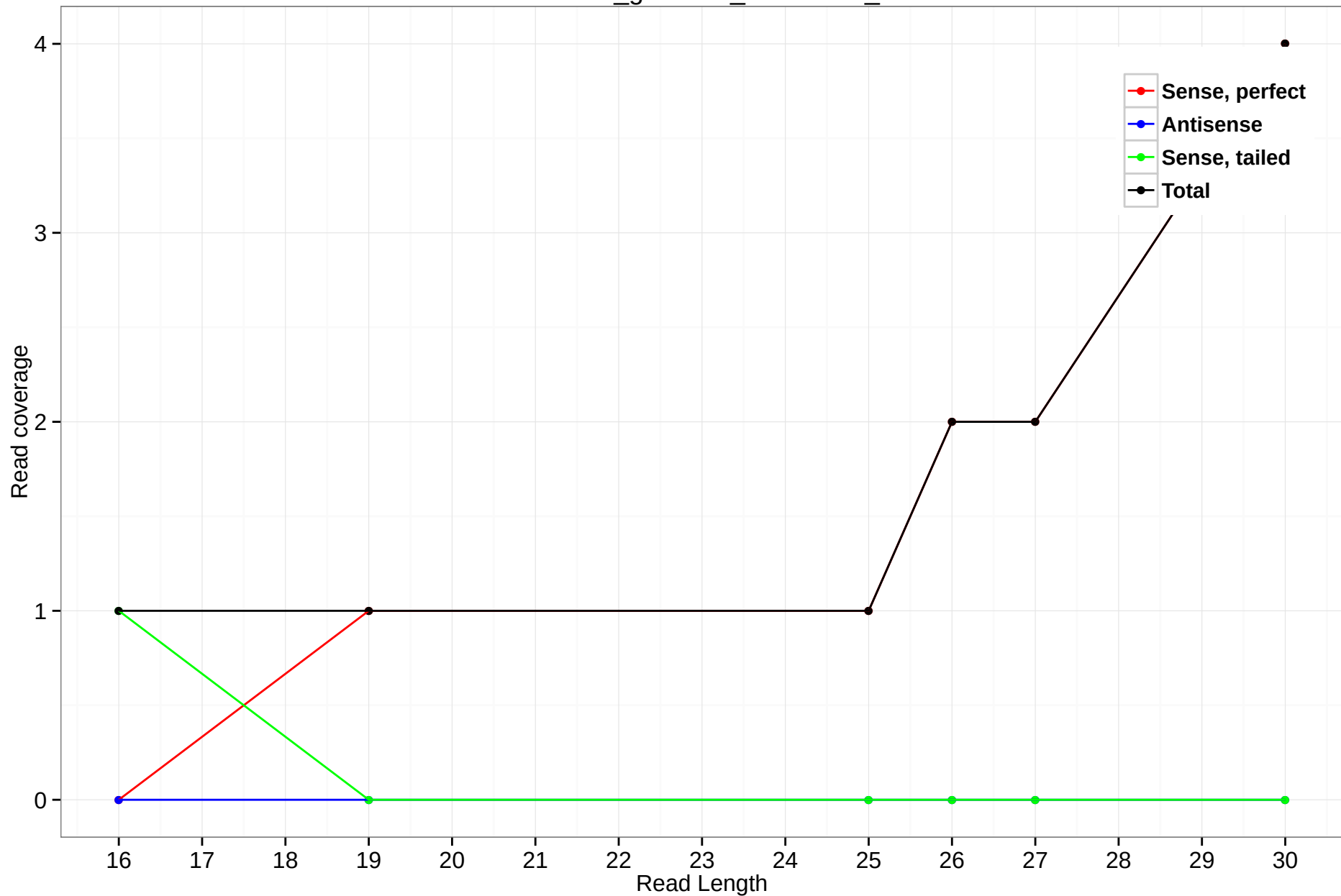
rheMac3_genscan_chr9.1140_2
