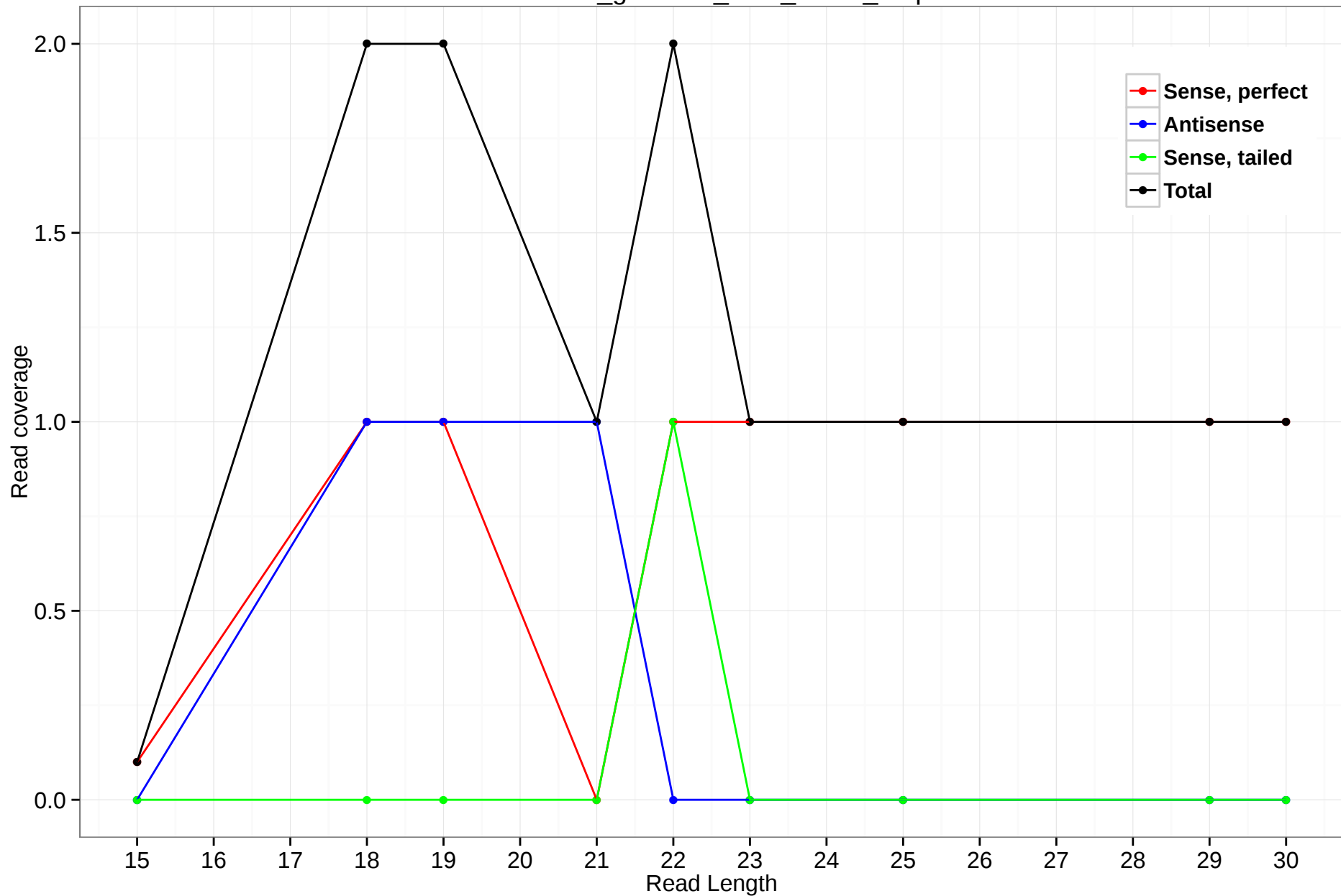
rheMac3_genscan_chr8_87.46_0.3p
