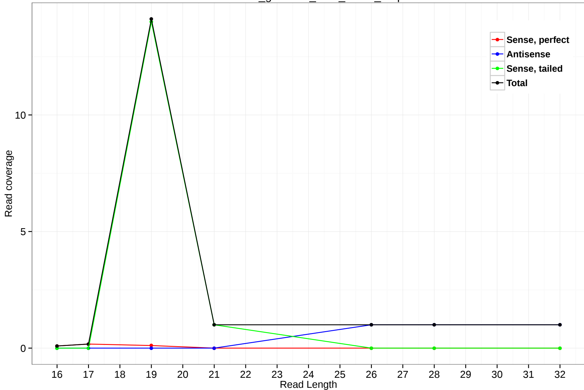
rheMac3_genscan_chr8_87.23_1.5p
