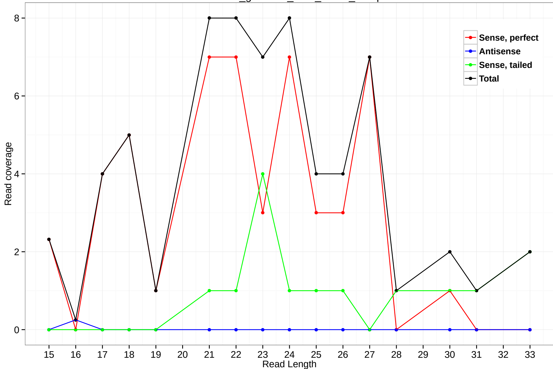
rheMac3_genscan_chr8_87.17_46.5p
