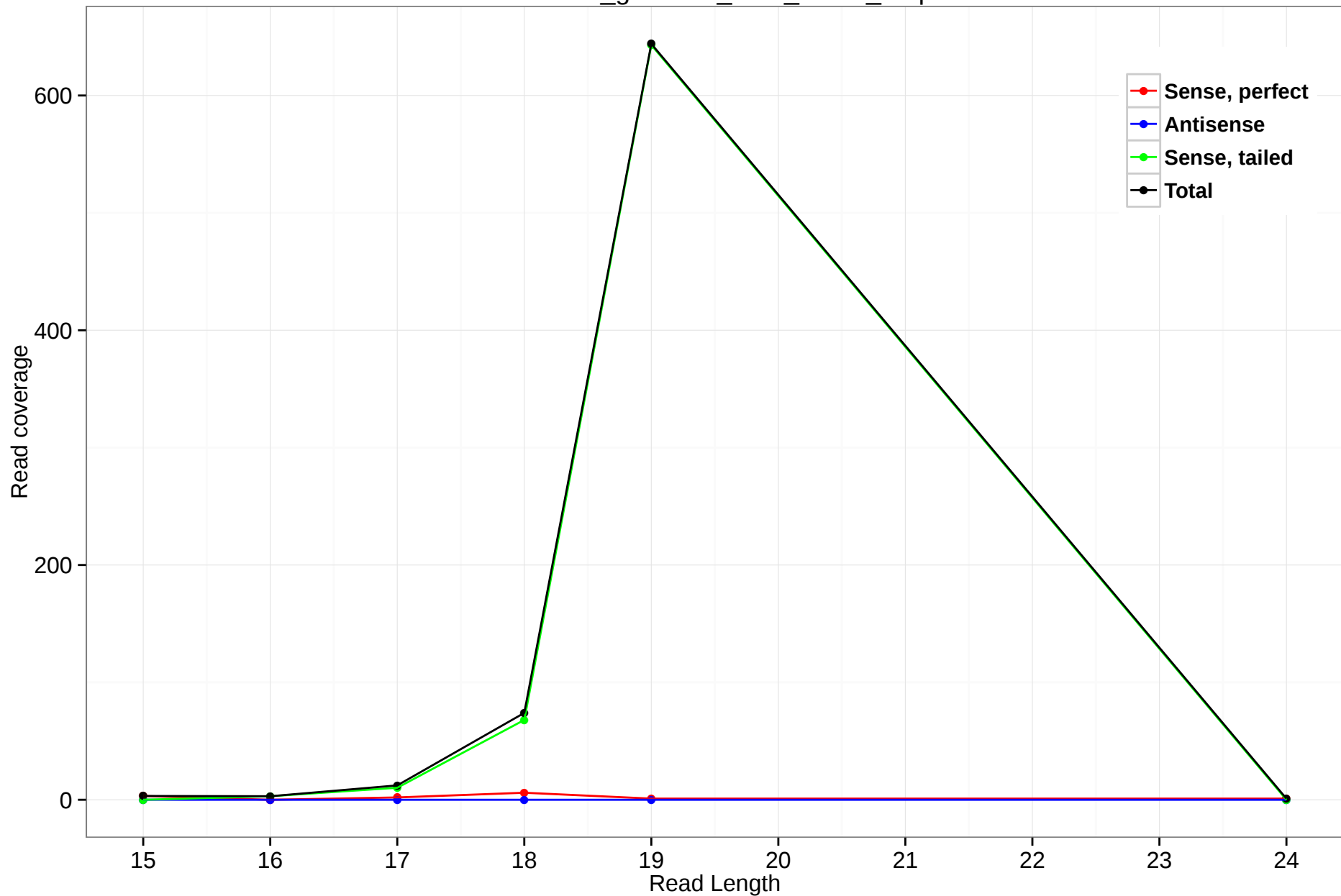
rheMac3_genscan_chr8_87.11_0.3p
