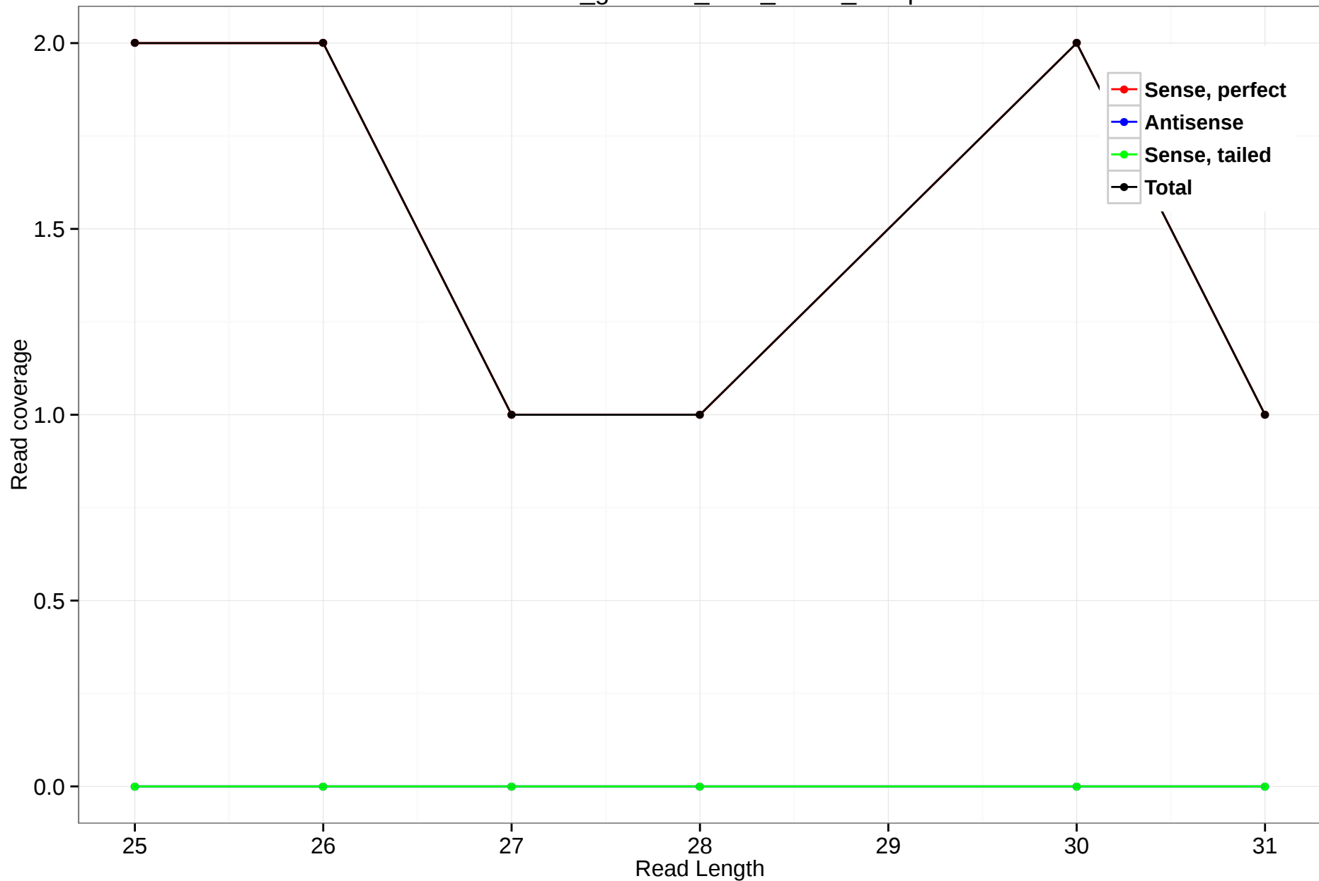
rheMac3_genscan_chr8_78.74_19.3p
