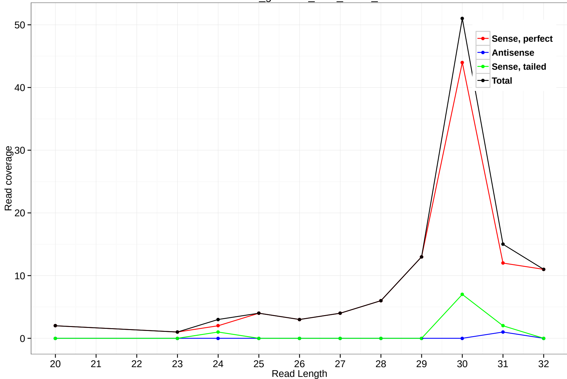
rheMac3_genscan_chr8_78.72_6
