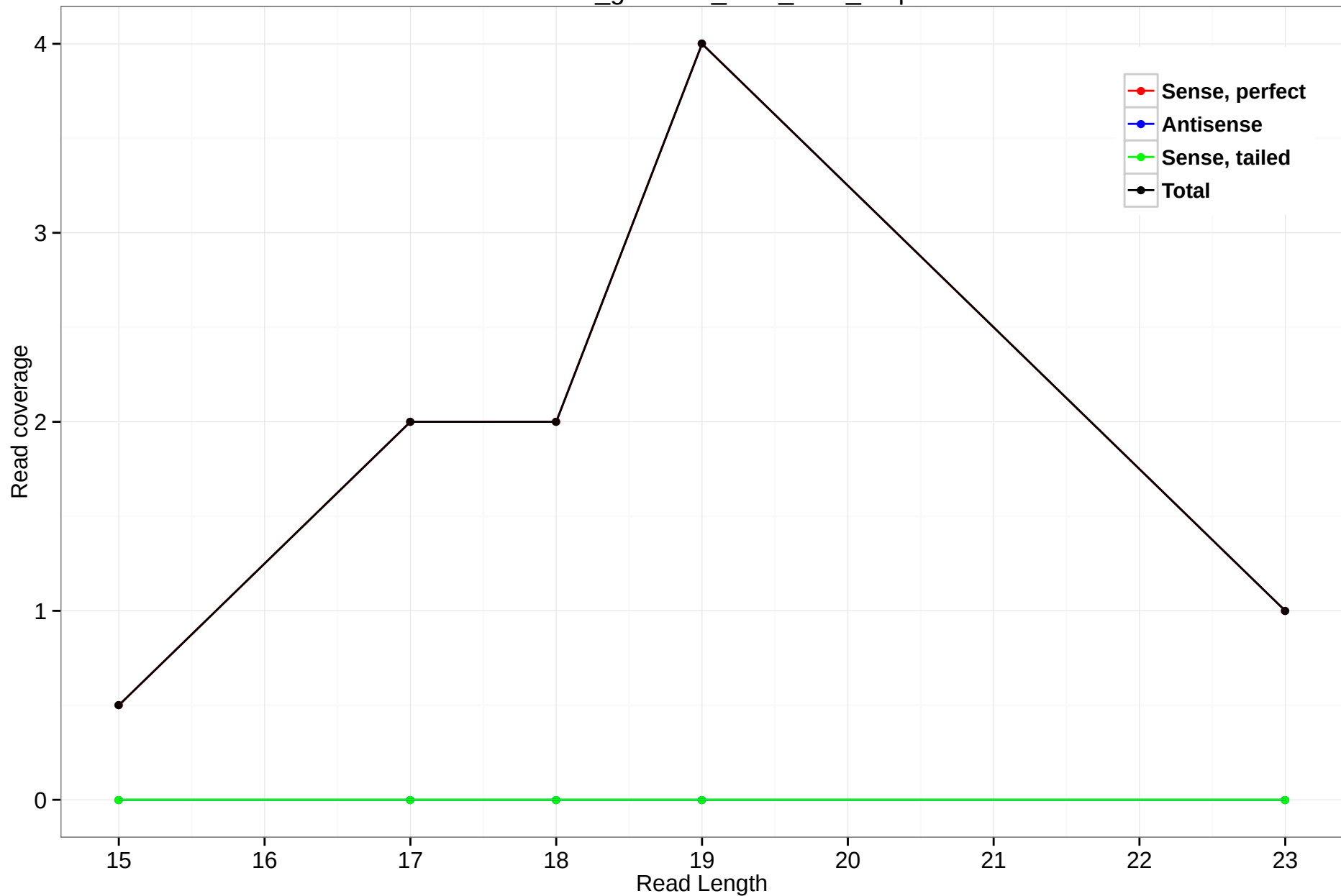
rheMac3_genscan_chr8_78.4_0.3p
