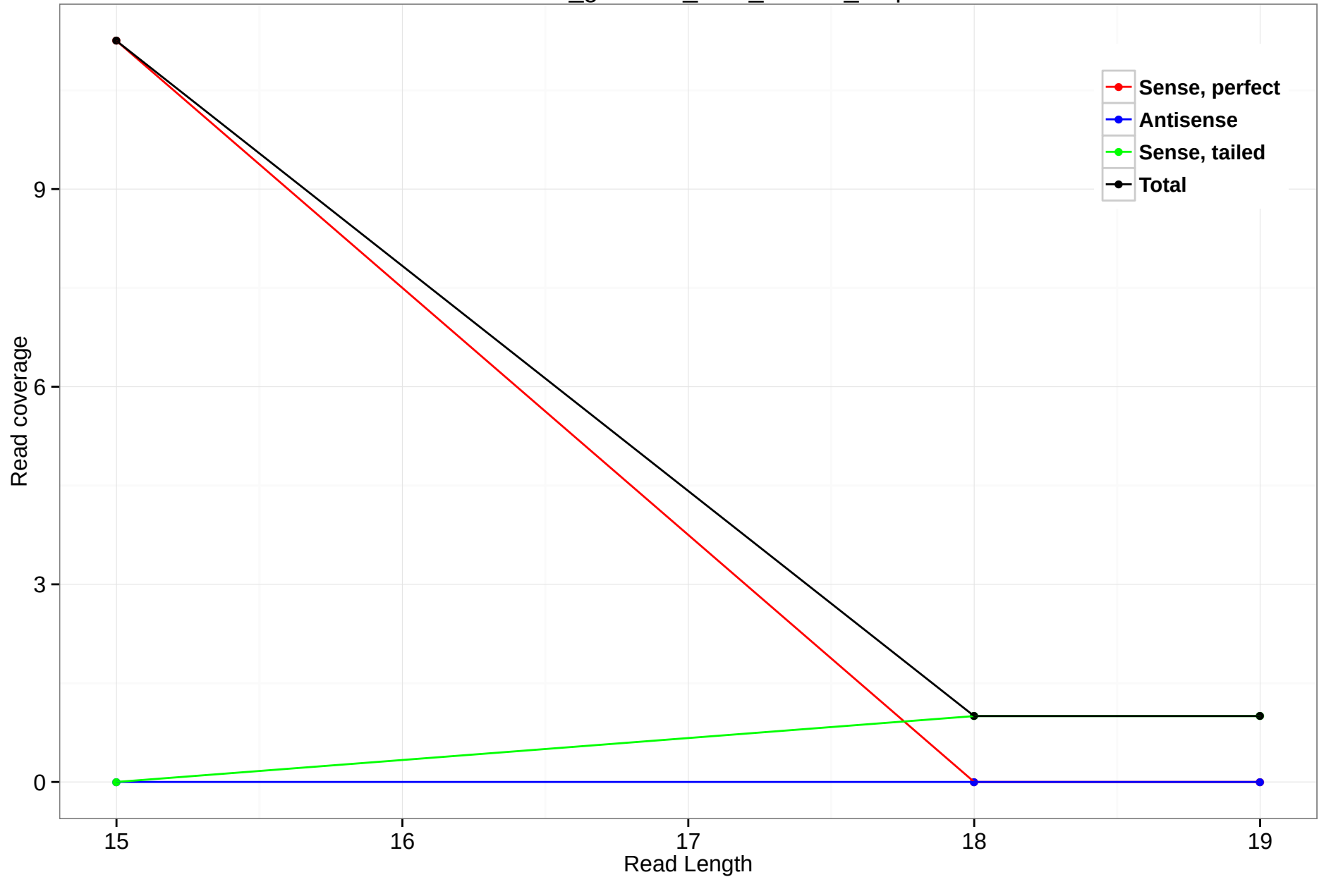
rheMac3_genscan_chr8_78.282_4.3p
