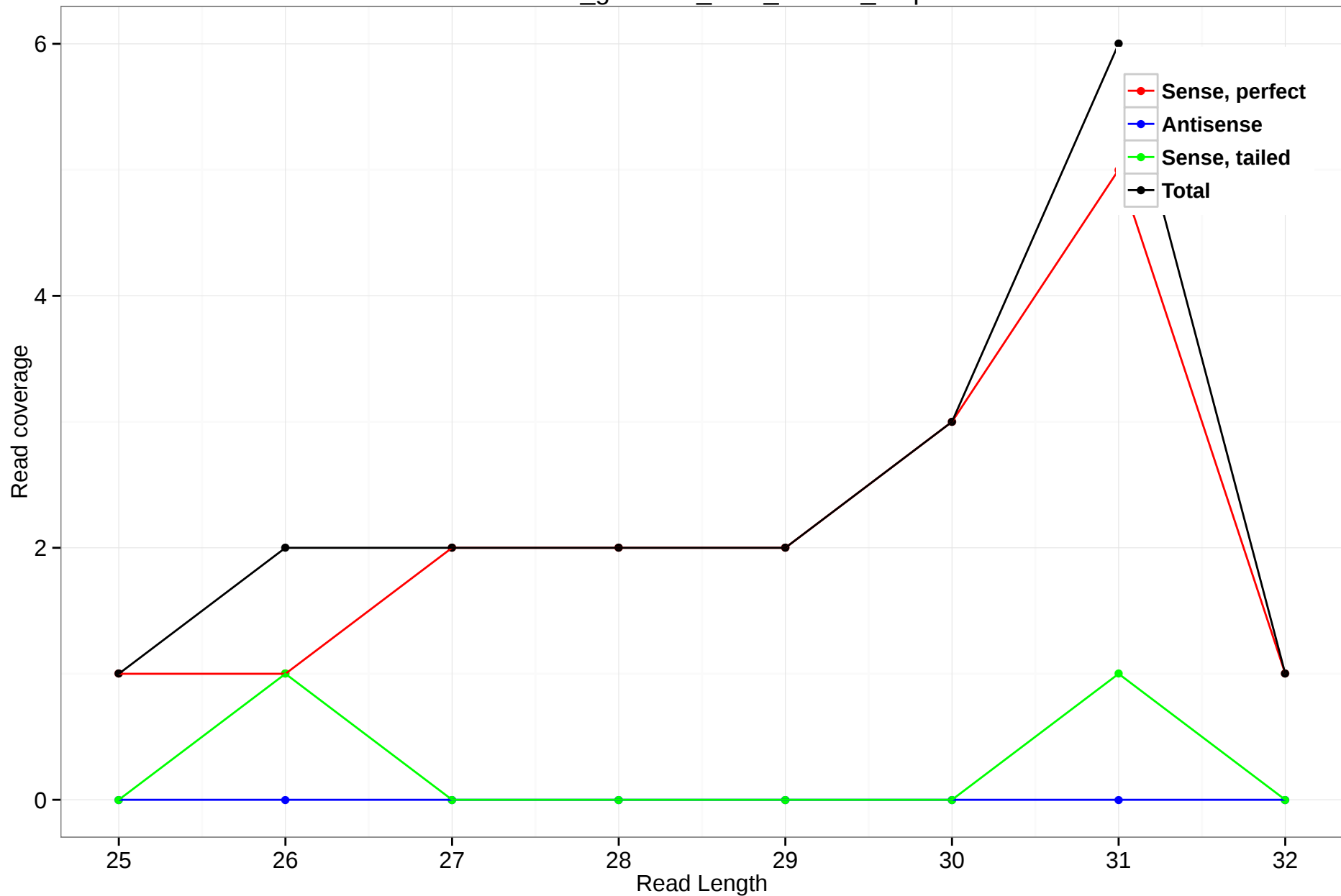
rheMac3_genscan_chr8_78.275_2.3p
