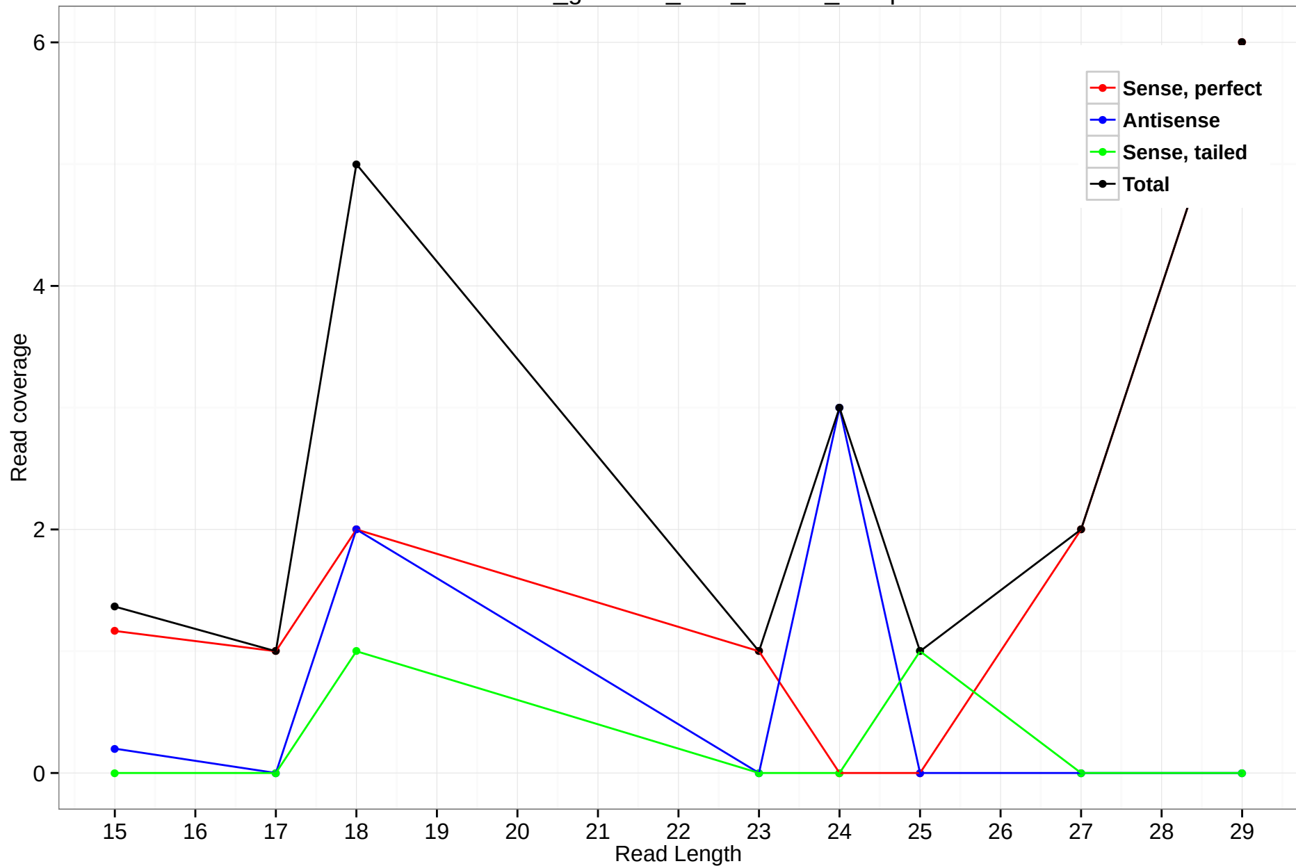
rheMac3_genscan_chr8_78.248_26.3p
