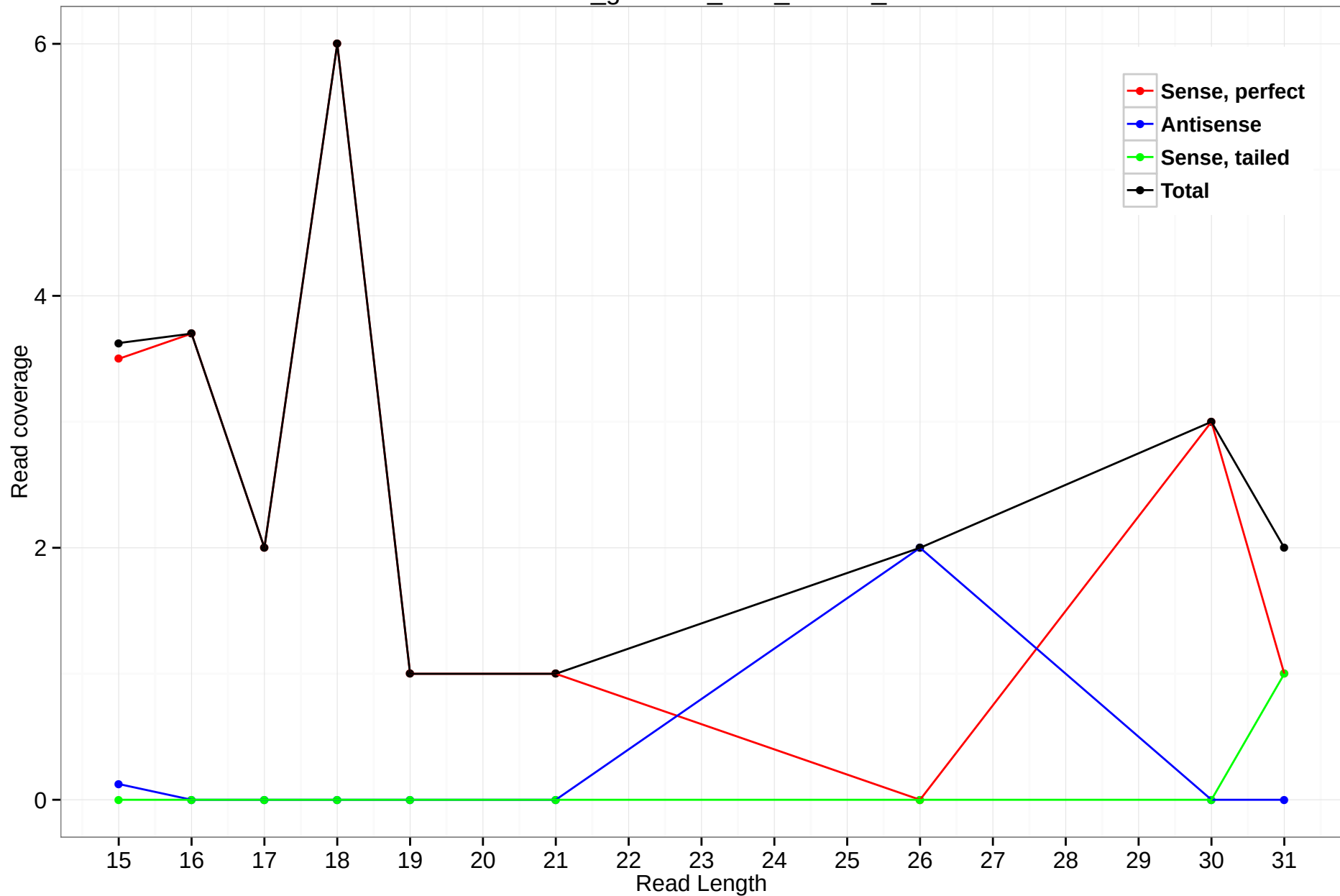
rheMac3_genscan_chr8_78.248_25
