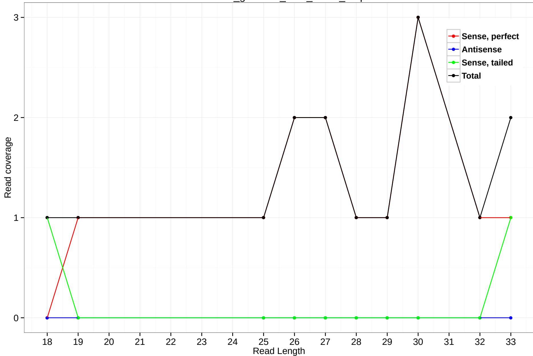
rheMac3_genscan_chr8_78.19_3.5p
