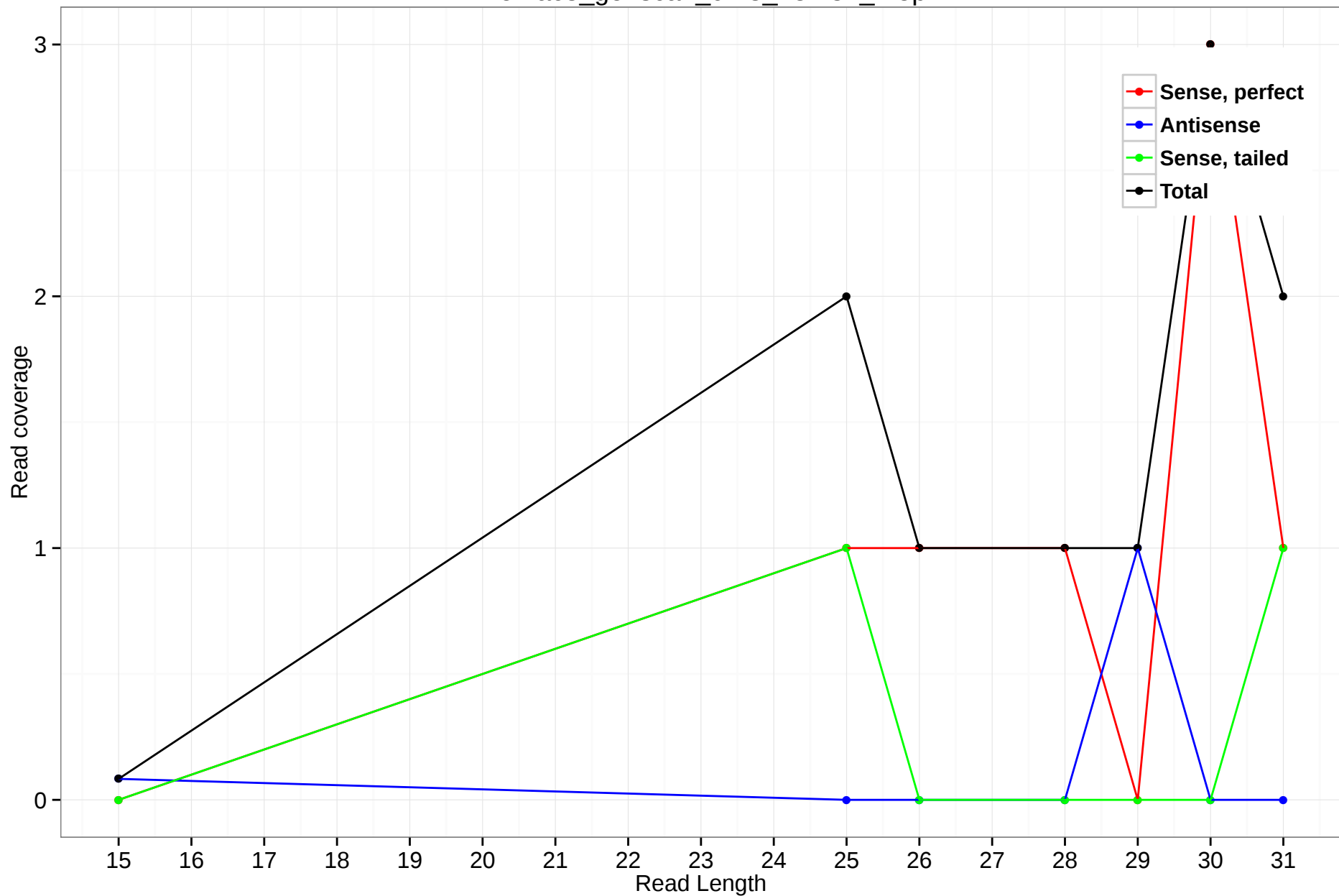
rheMac3_genscan_chr8_78.132_2.5p
