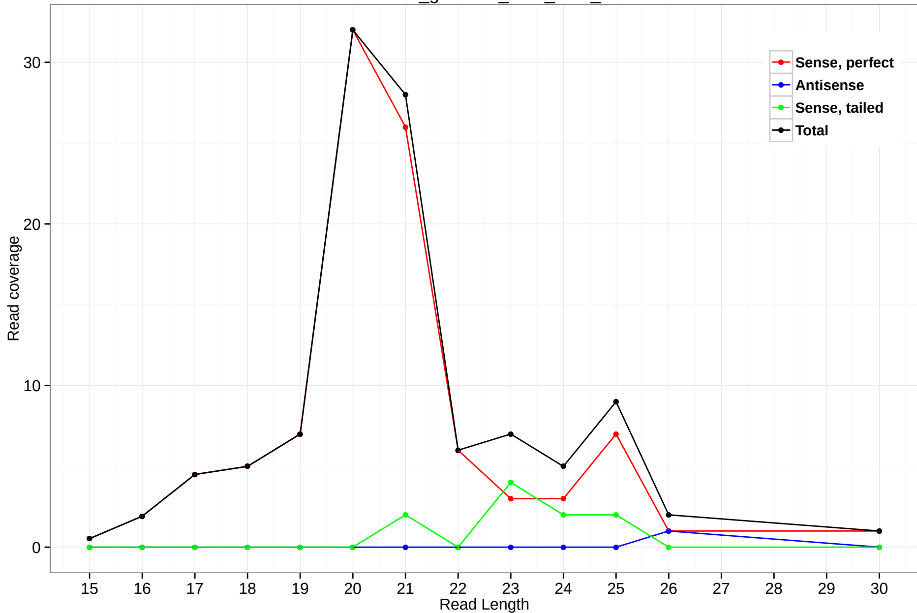
rheMac3_genscan_chr8_73.7_49
