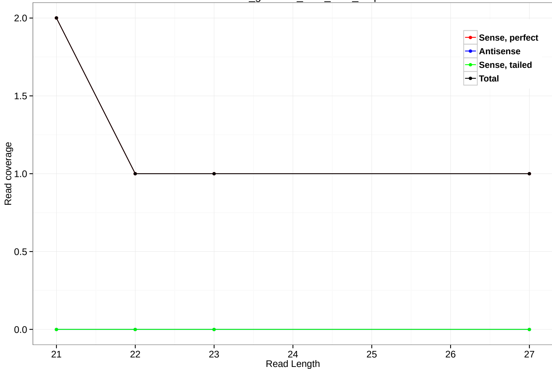
rheMac3_genscan_chr8_73.6_6.5p
