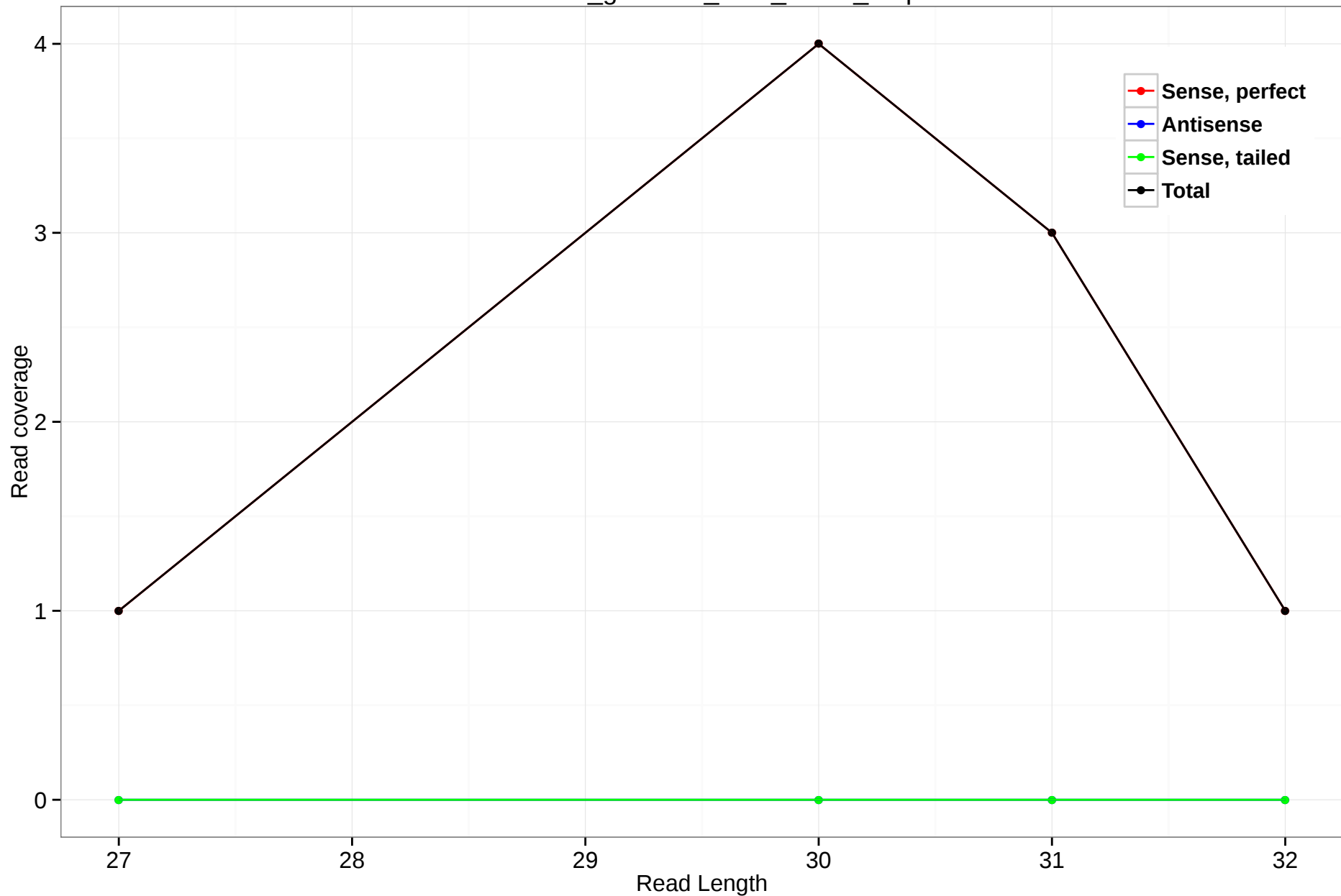
rheMac3_genscan_chr8_73.12_8.5p
