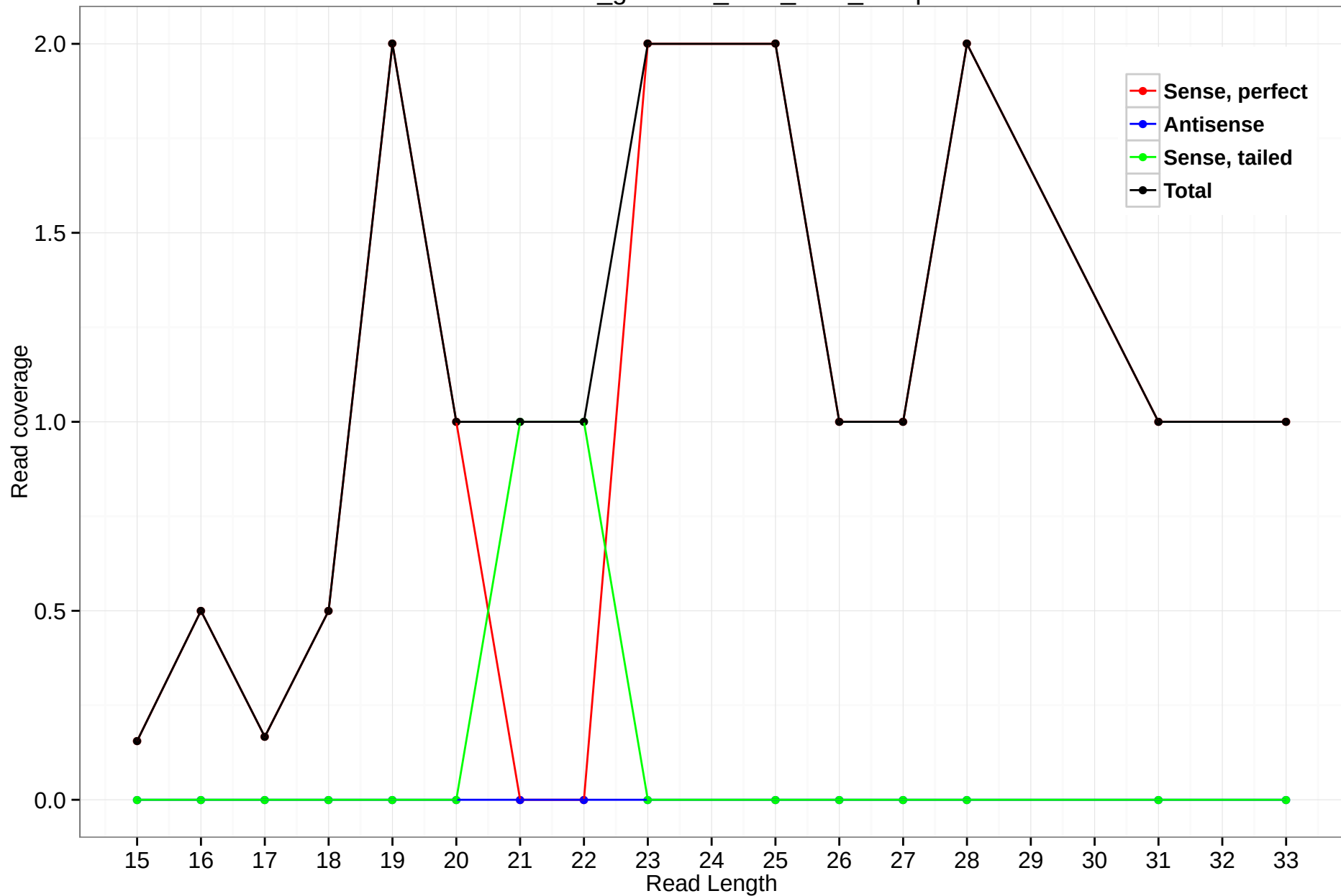
rheMac3_genscan_chr8_69.8_10.5p
