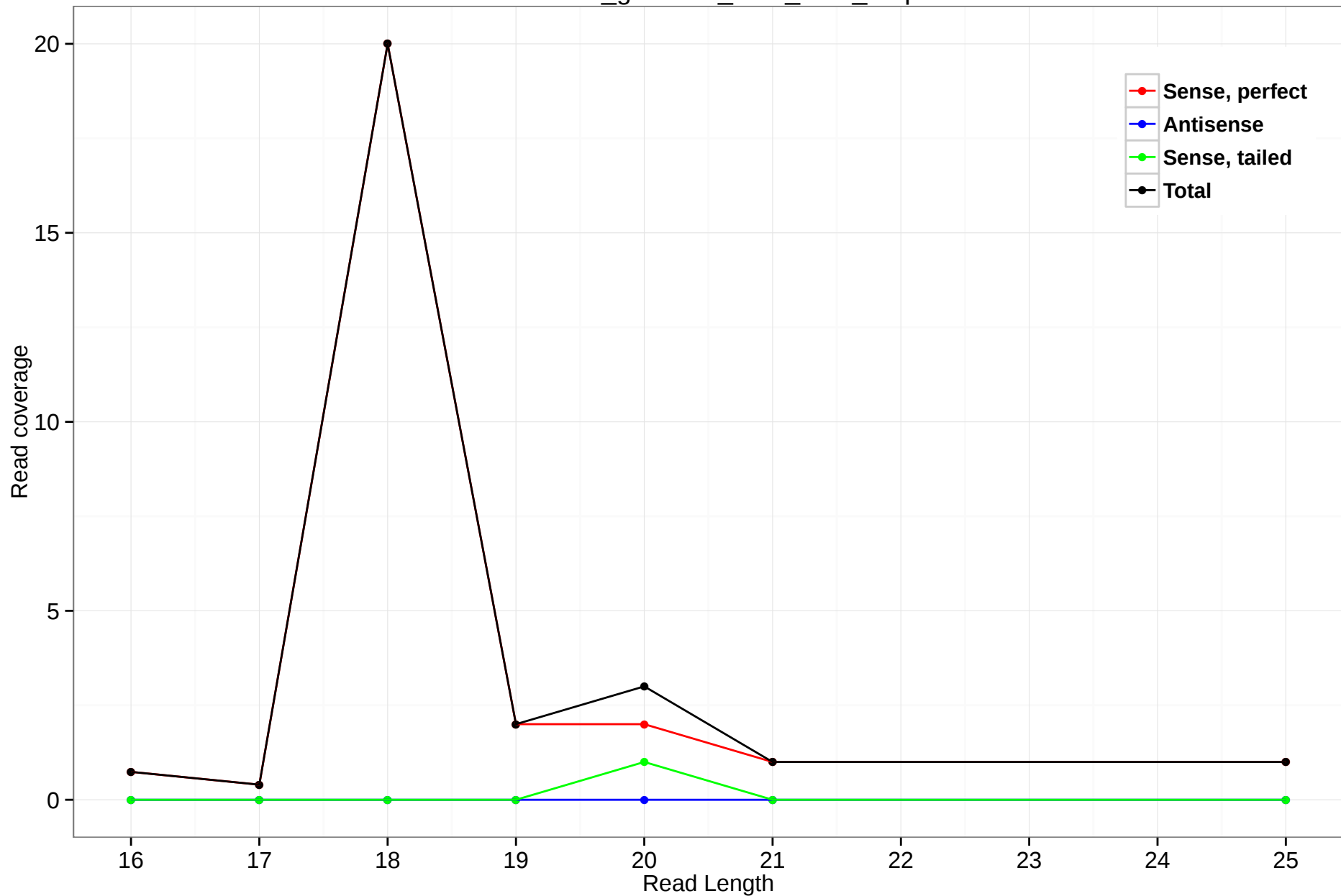
rheMac3_genscan_chr8_69.4_1.5p
