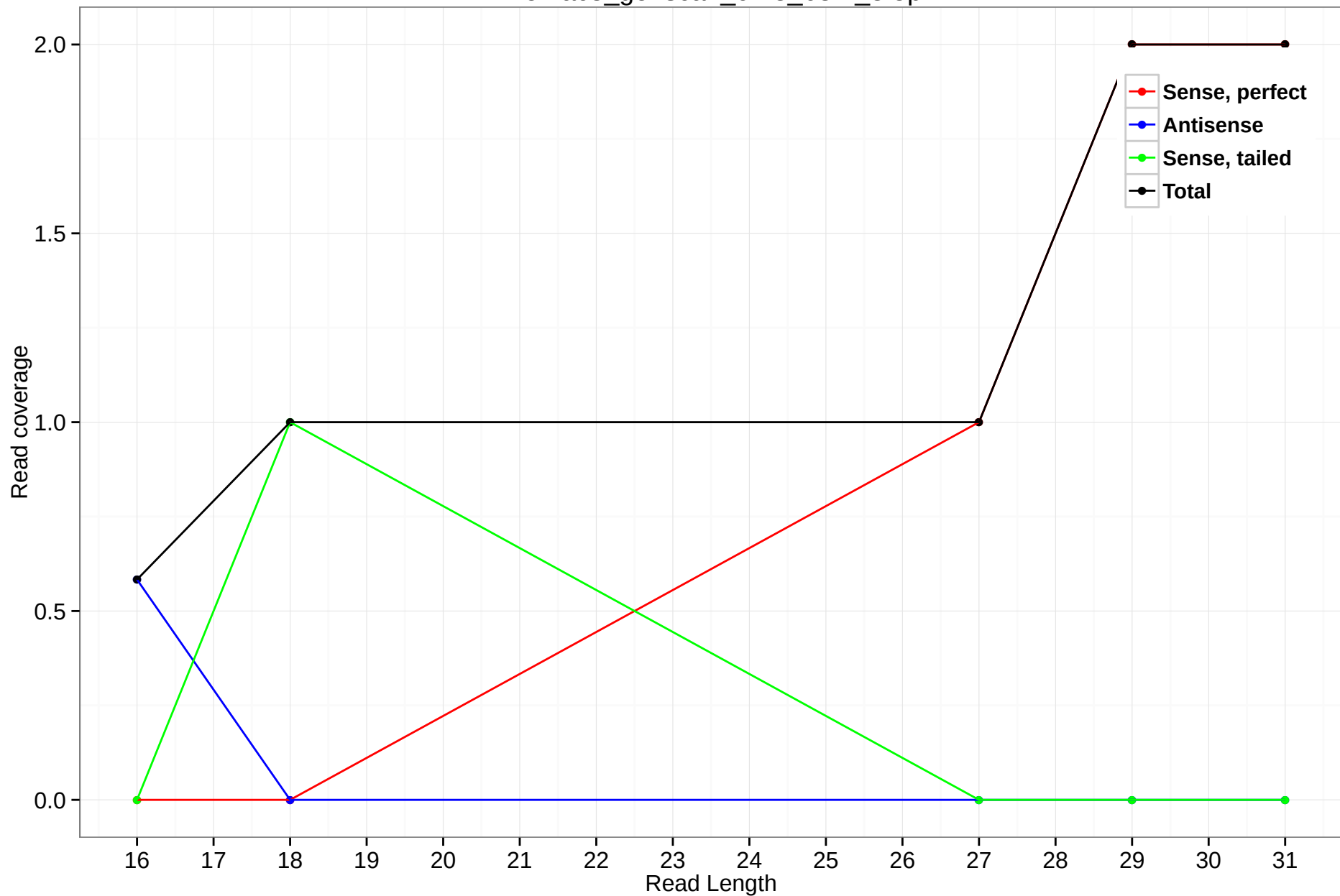
rheMac3_genscan_chr8_63.4_3.5p
