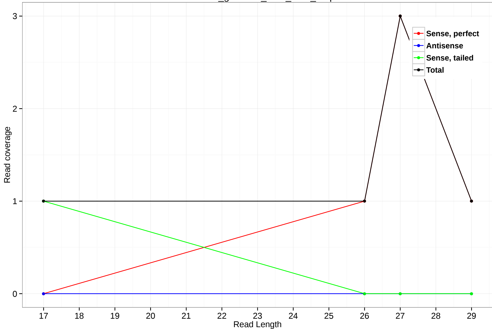
rheMac3_genscan_chr8_55.8_2.5p
