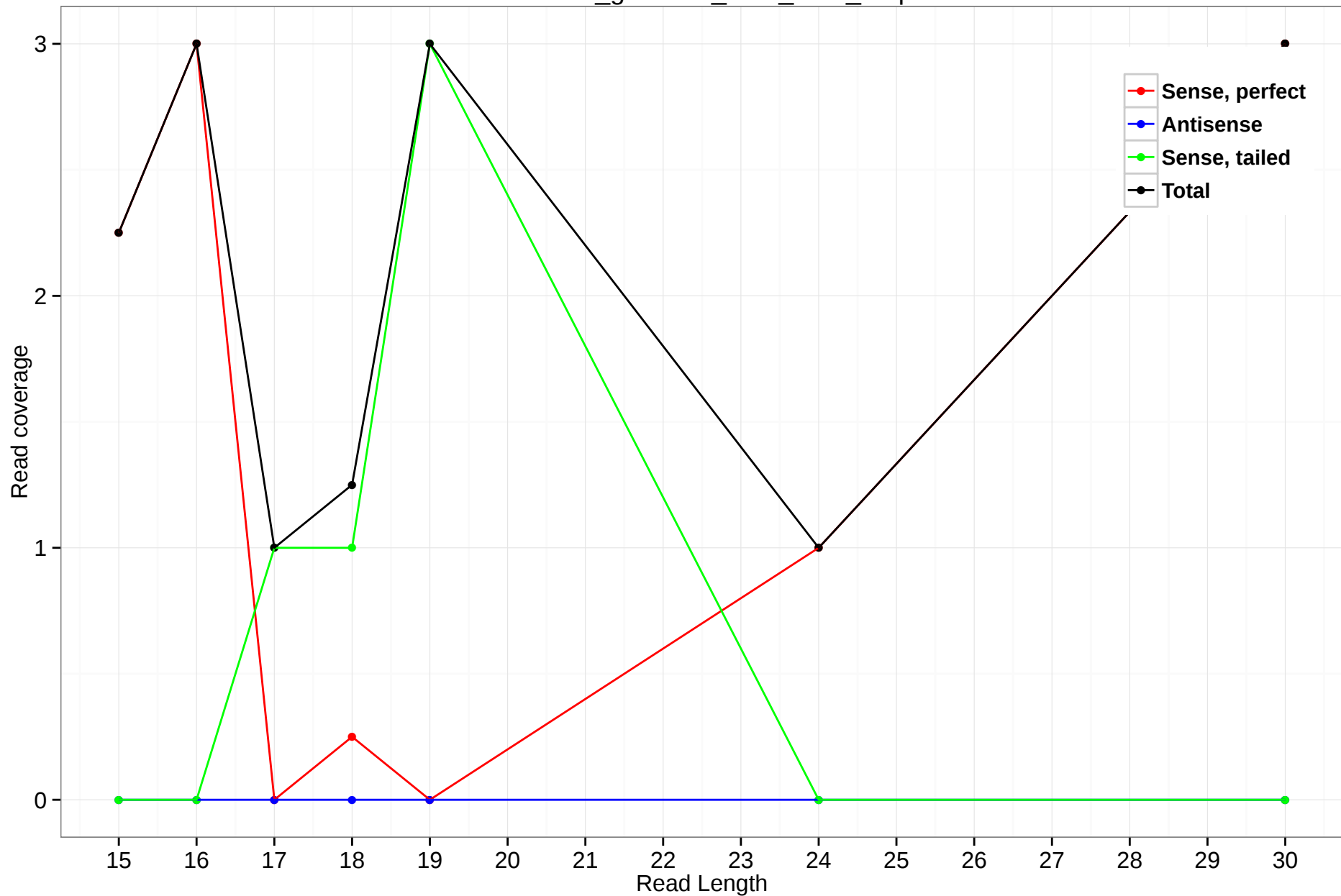
rheMac3_genscan_chr8_53.4_5.5p
