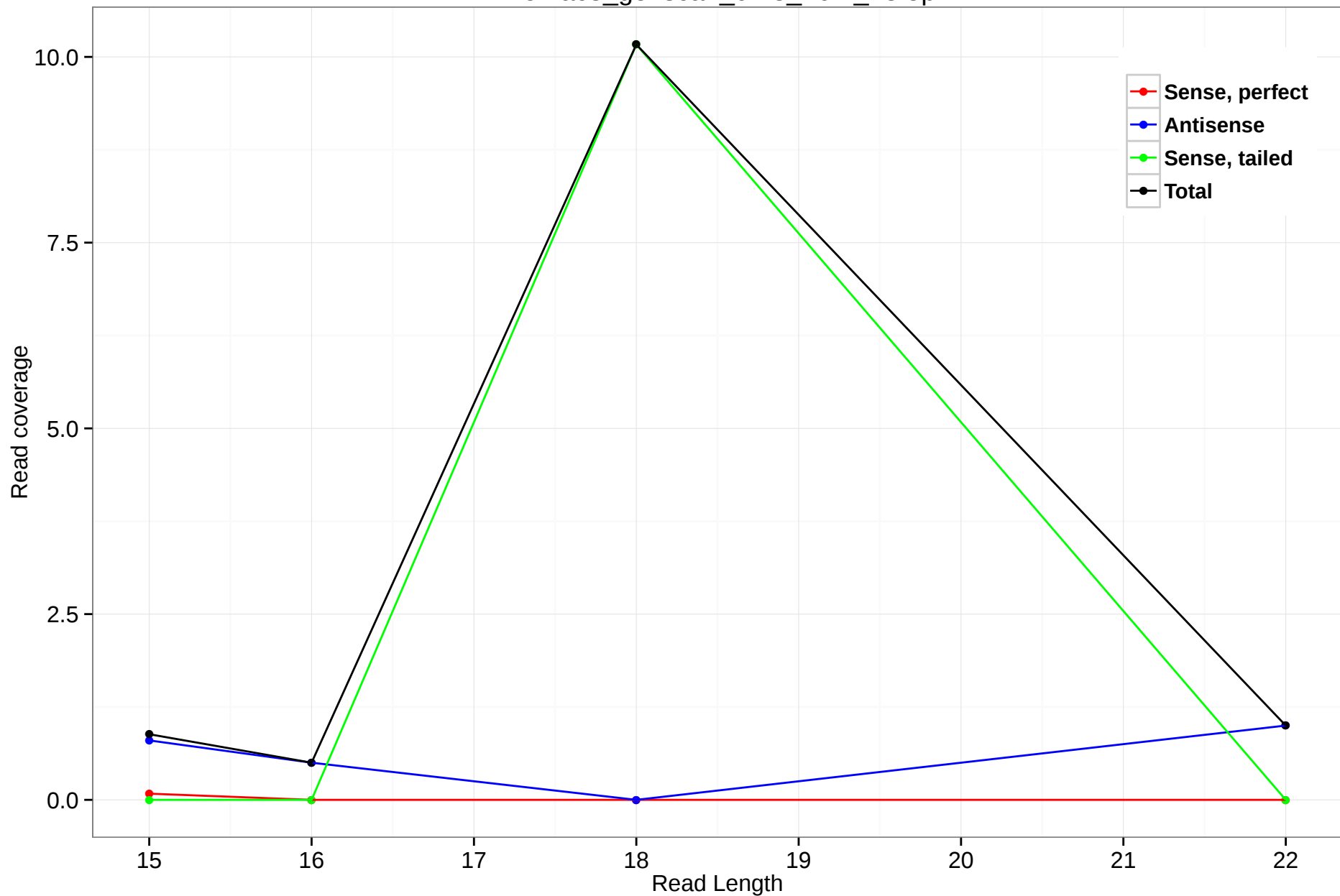
rheMac3_genscan_chr8_26.1_13.5p
